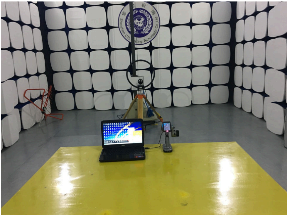
Radiated emission 30M~1G
