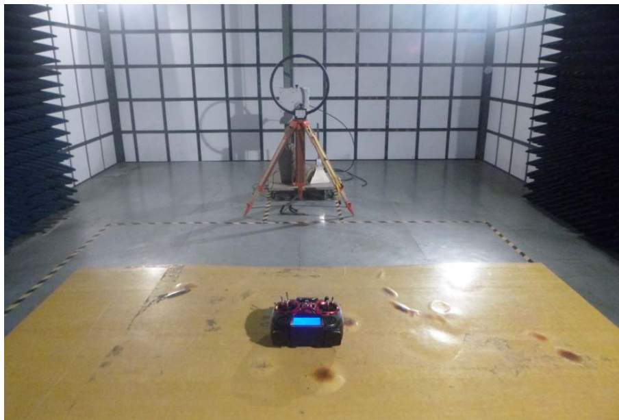
Radiated emission below 30M
