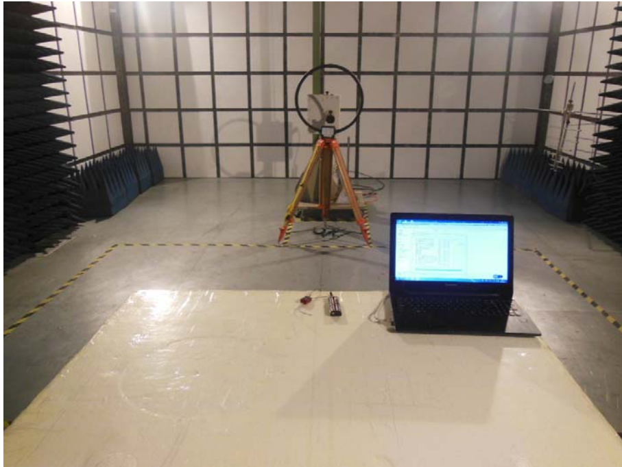
Radiated emission below 30M
