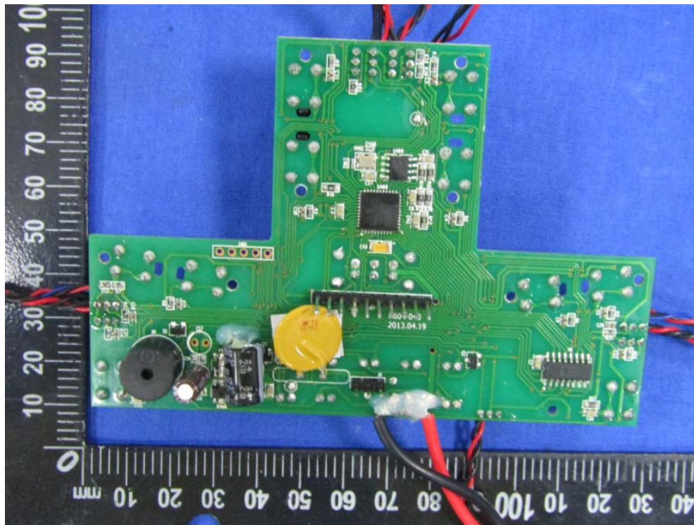
EUT – RF Module View
