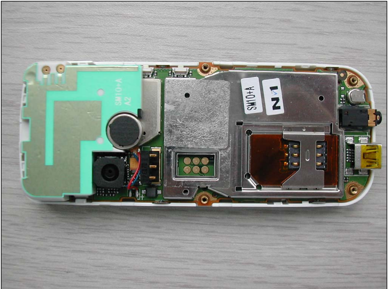
With Shields
