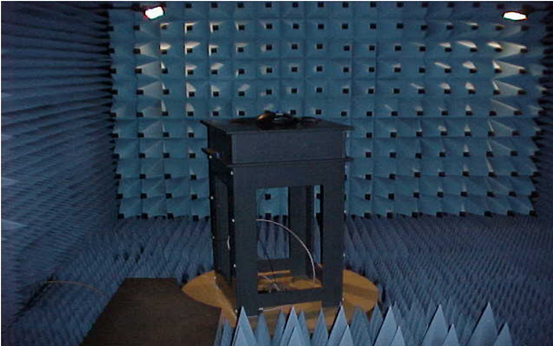
Radiated spurious emission 1-26 GHz
