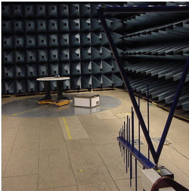
Radiated spurious emission 30-1000 MHz
