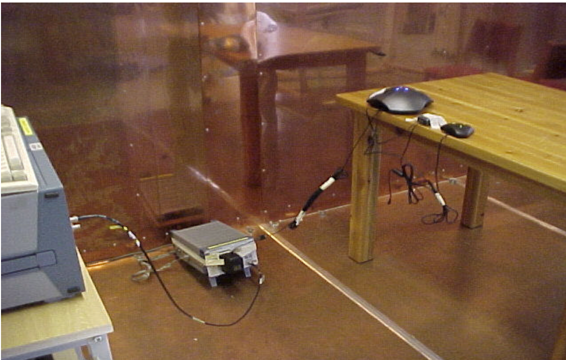
Conducted disturbance voltage in the frequency range 0,15 - 30 MHz
