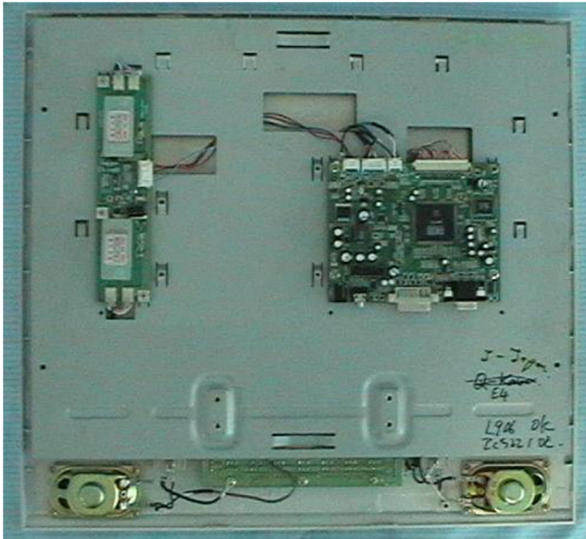
L1911MN PCB without shield
