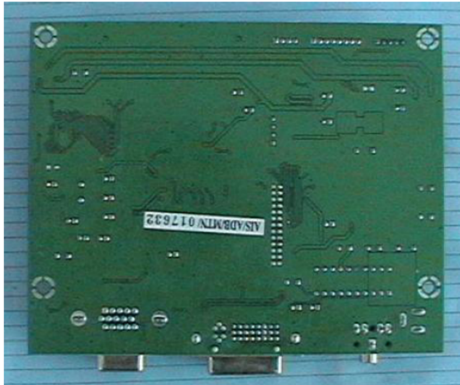
L1711MN/L1911MN Common PCB – Solder Side
