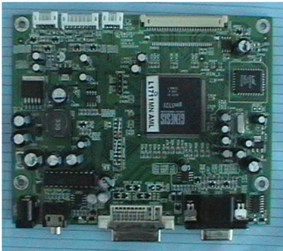
L1711MN/L1911MN Common PCB – Component Side
