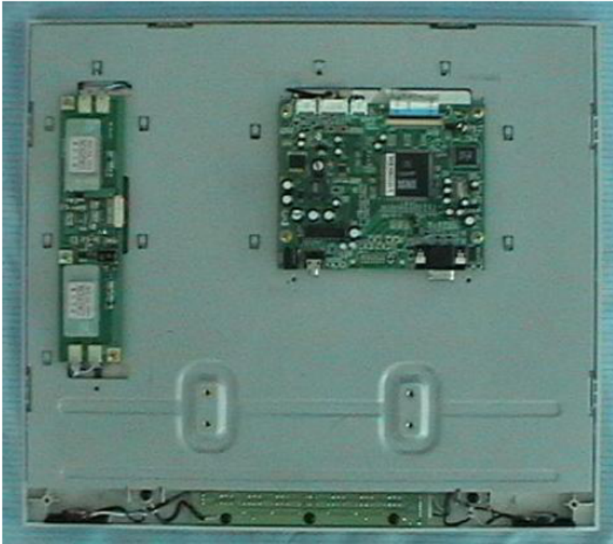
L1711MN PCB without shield
