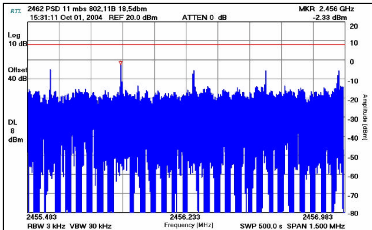
PLOT 4-10: POWER SPECTRAL DENSITY: CHANNEL 11 (2462 MHz – 11 MB/S)
