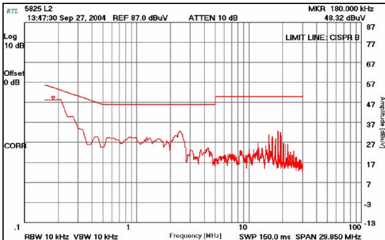
PLOT 5-14: CONDUCTED TEST DATA; MODE TX, CHANNEL 13, HOT SIDE (LINE 2)
