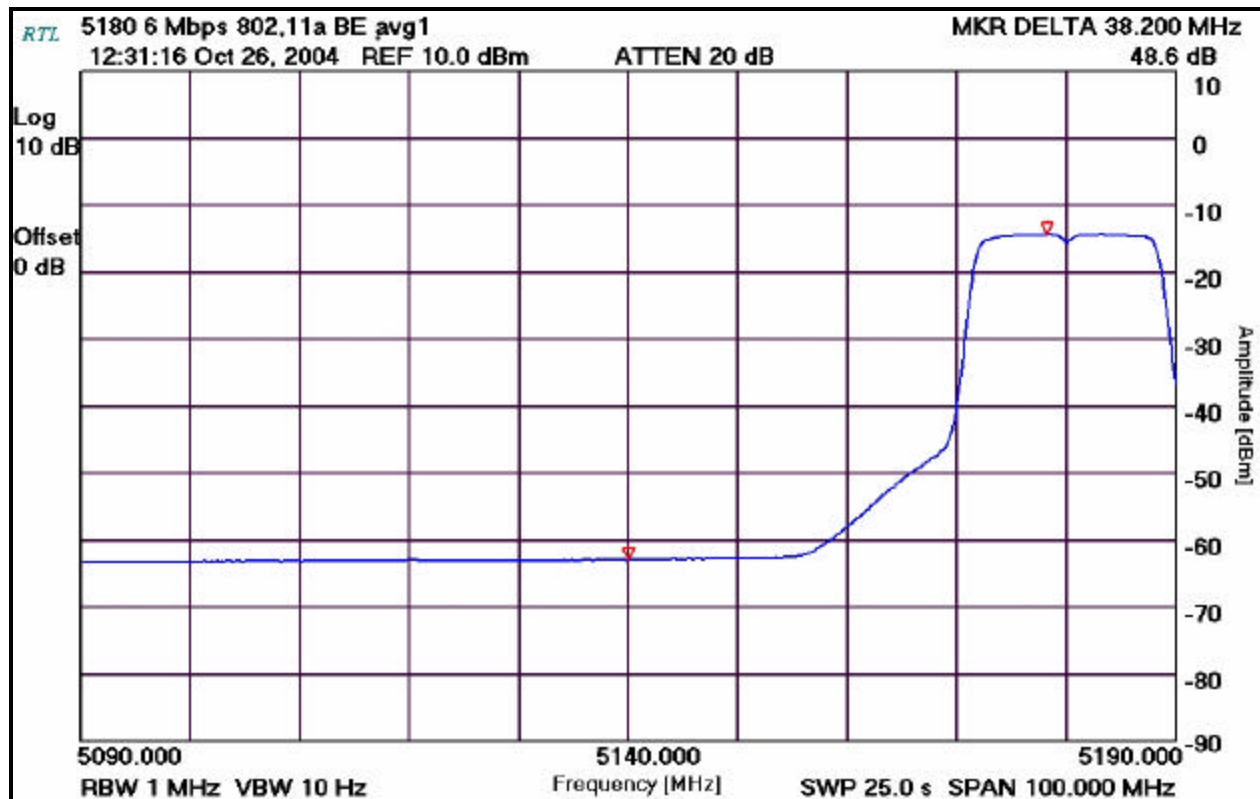
PLOT 6-12: LOWER BAND EDGE: AVERAGE MEASUREMENT CHANNEL 1 (TX FREQUENCY: 5180 MHZ)
