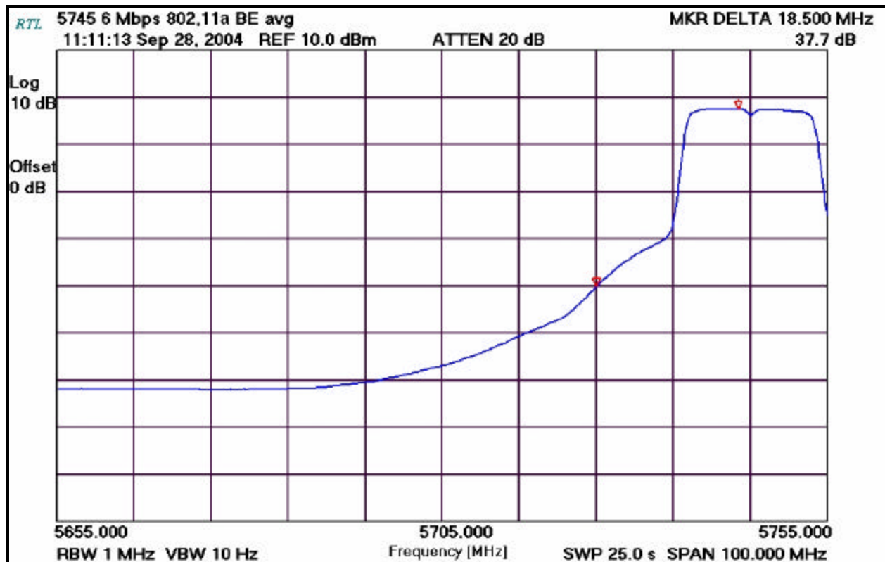
PLOT 7-8: LOWER BAND EDGE: AVERAGE MEASUREMENT CHANNEL 9 (TX FREQUENCY: 5745 MHz – 6 MB/S)
