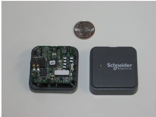
EUT PCB in case (top)
