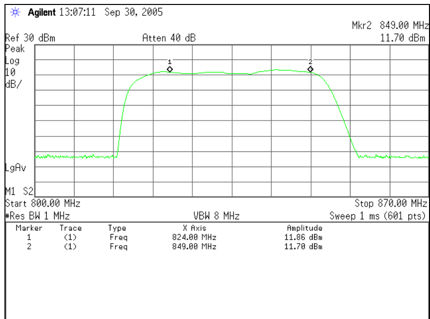
Figure 7.6-1: Frequency Response Uplink
