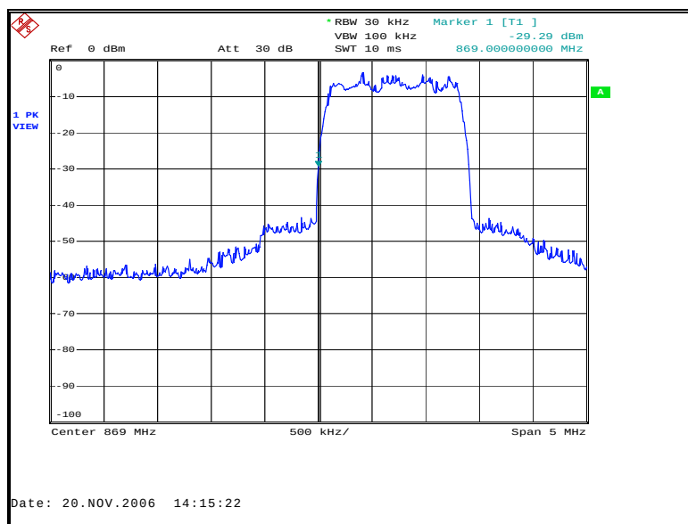
Figure 81: Band-Edge Downlink CDMA Low Channel
