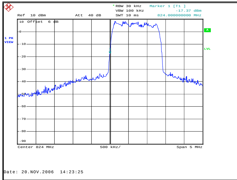
Figure 75: Band-Edge Uplink CDMA Low Channel
