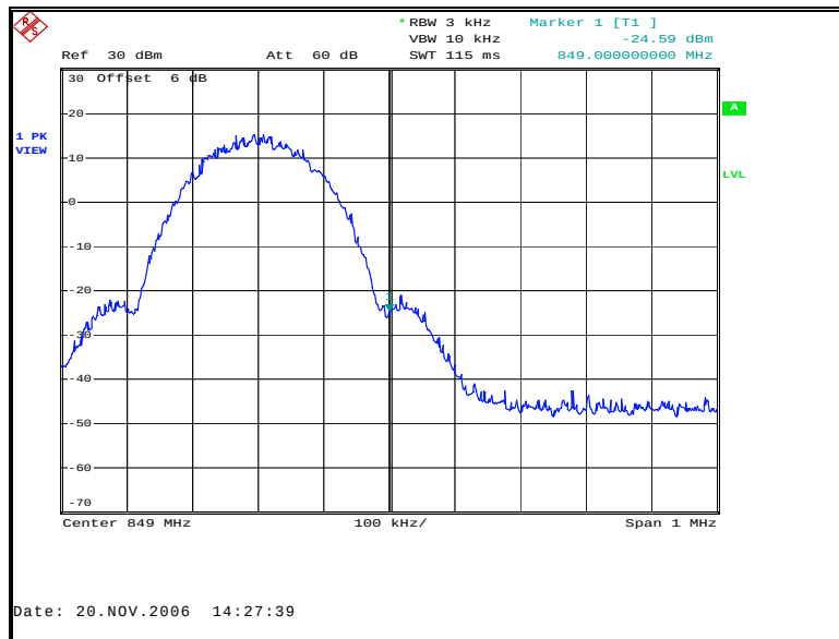
Figure 80: Band-Edge Uplink GSM High Channel
