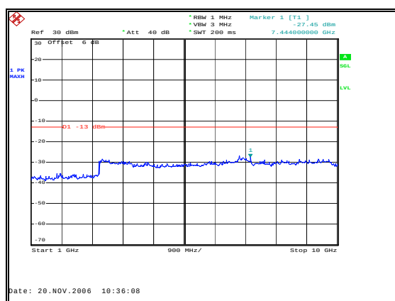
Figure 42: Spurious Emissions - Uplink GSM Low Channel – 1 to 10 GHz
