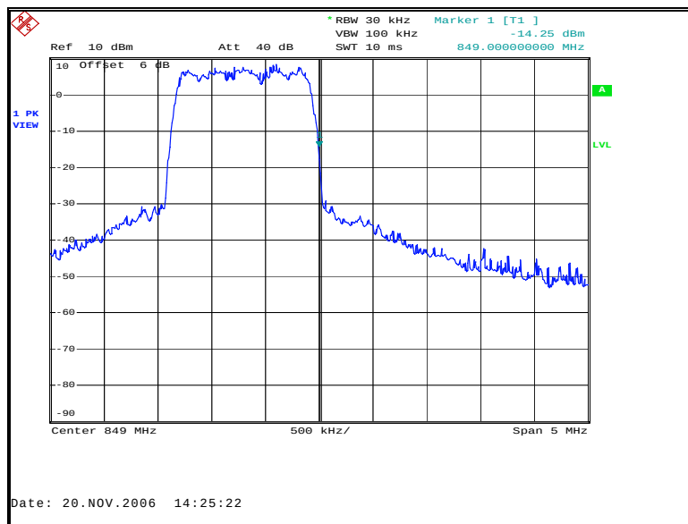
Figure 76: Band-Edge Uplink CDMA High Channel
