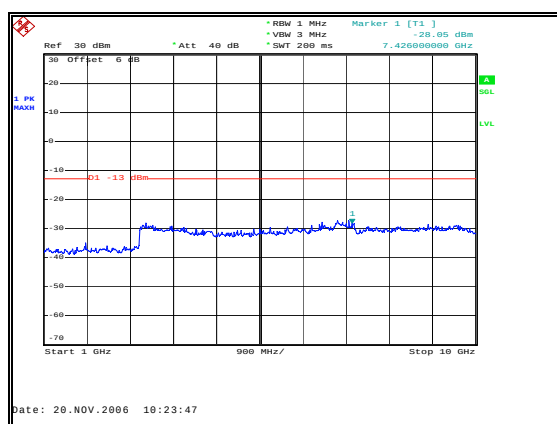
Figure 31: Spurious Emissions - Uplink TDMA Mid Channel – 1 to 10 GHz
