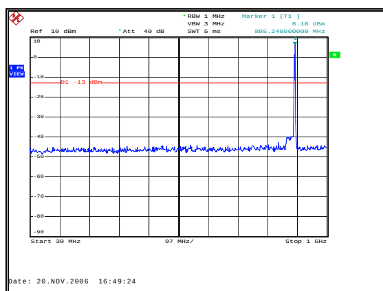
Figure 67: Spurious Emissions - Downlink CW High Channel – Inter-modulation - 30 MHz to 1 GHz
