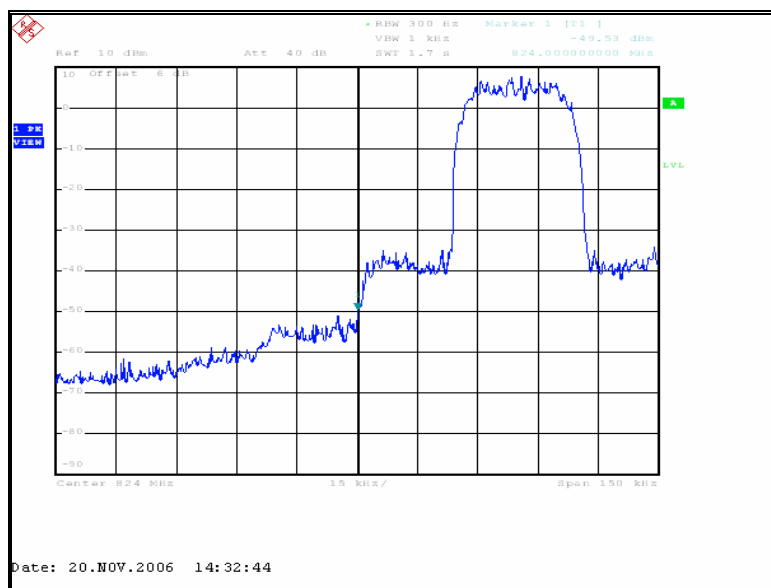
Figure 77: Band-Edge Uplink TDMA Low Channel
