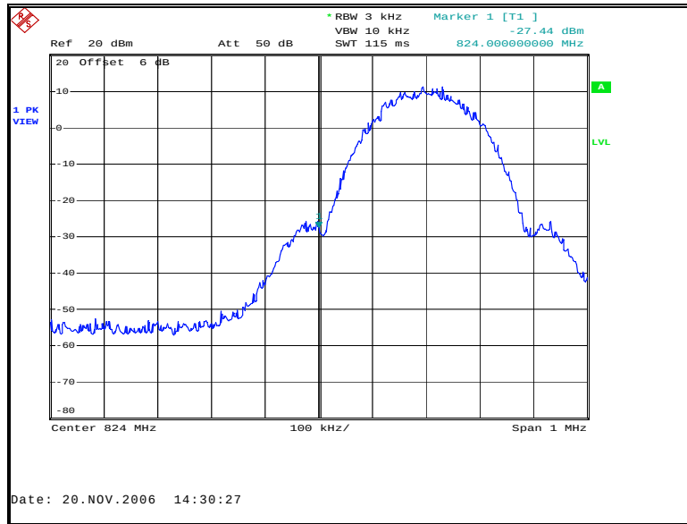
Figure 79: Band-Edge Uplink GSM Low Channel
