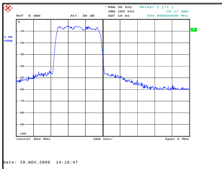
Figure 82: Band-Edge Downlink CDMA High Channel
