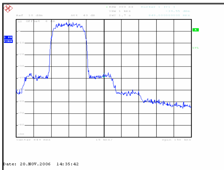
Figure 78: Band-Edge Uplink TDMA High Channel
