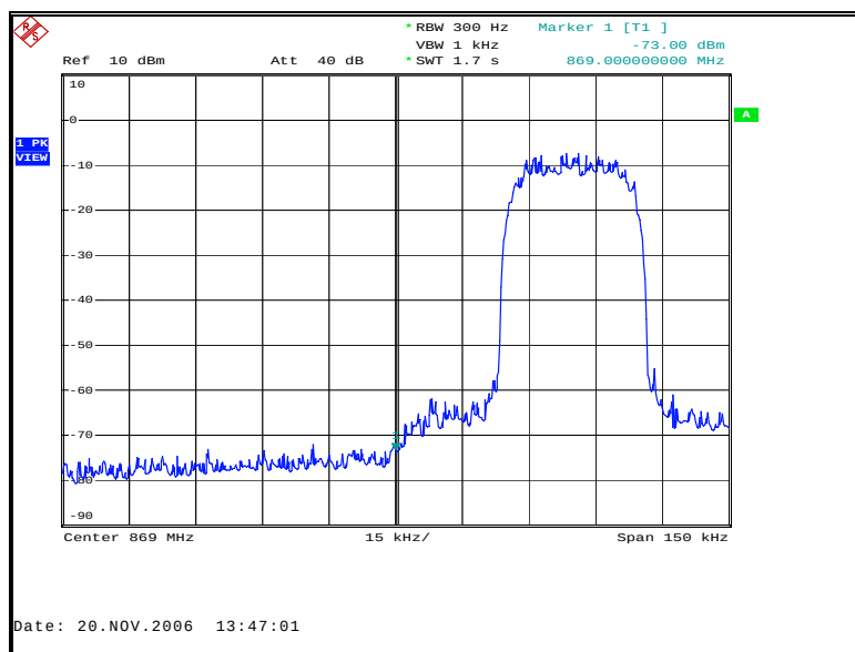
Figure 83: Band-Edge Downlink TDMA Low Channel
