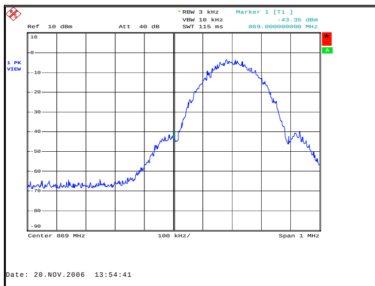
Figure 85: Band-Edge Downlink GSM Low Channel
