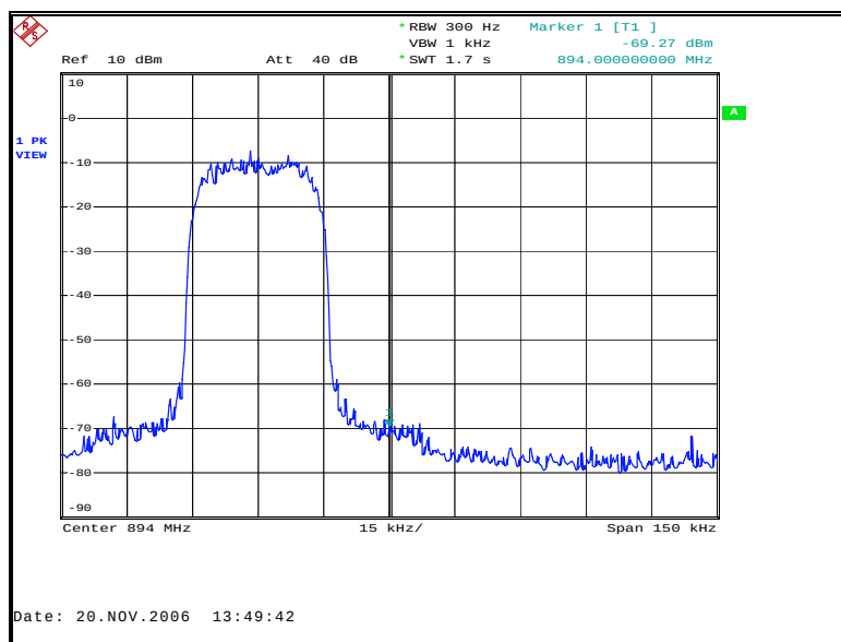
Figure 84: Band-Edge Downlink TDMA High Channel
