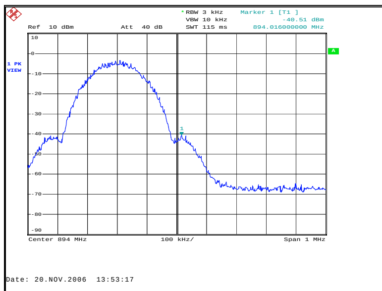
Figure 86: Band-Edge Downlink GSM High Channel
