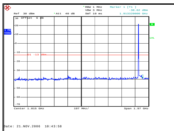
Figure 36: Spurious Emissions - Uplink CW Low Channel – Inter-modulation - 30 MHz to 2 GHz
