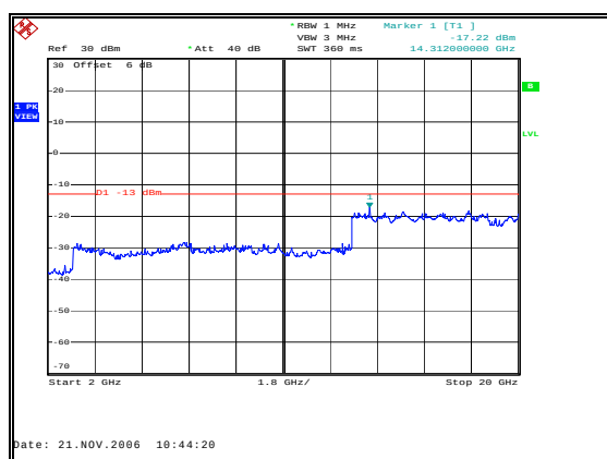
Figure 37: Spurious Emissions - Uplink CW Low Channel – Inter-modulation - 2 GHz to 20 GHz
