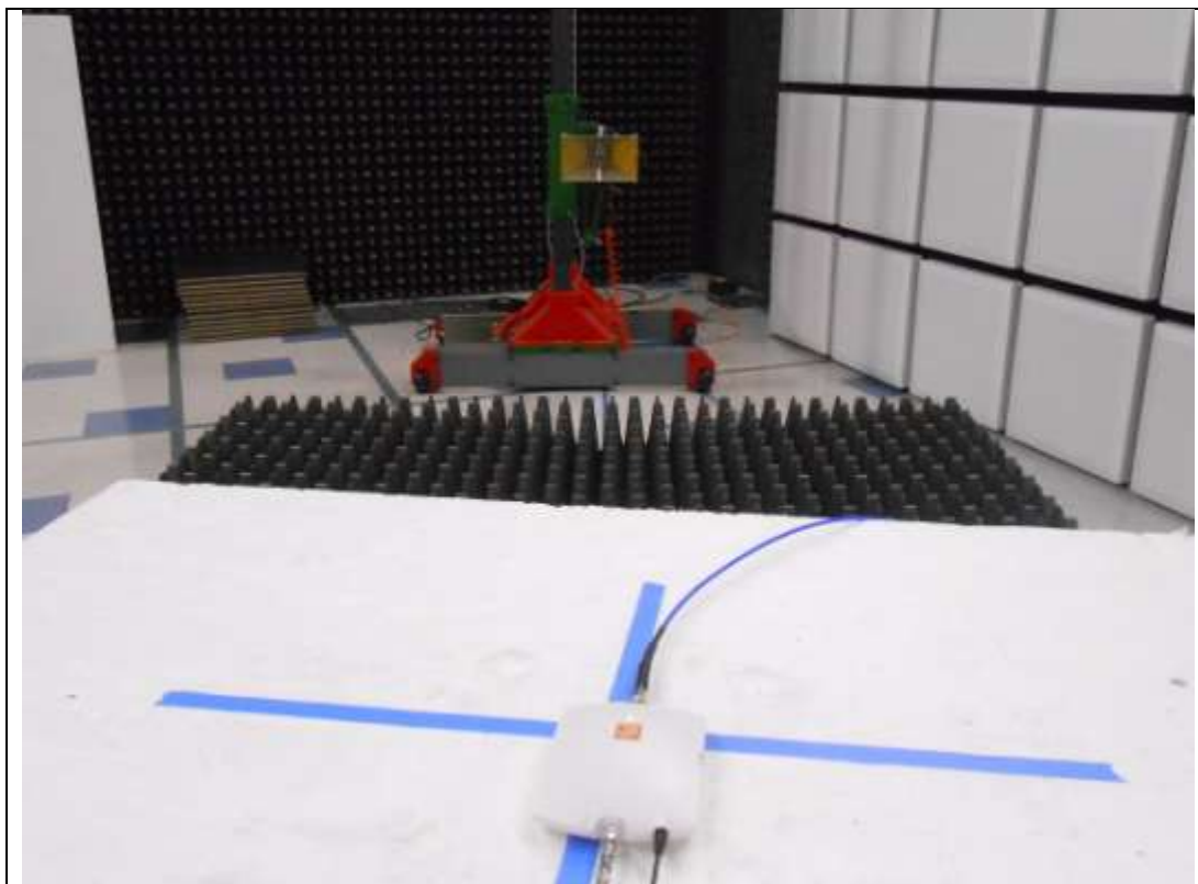
RF Radiated #2
