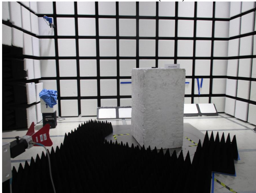
RADIATED EMISSIONS ABOVE 1000 MHz (BACK)
