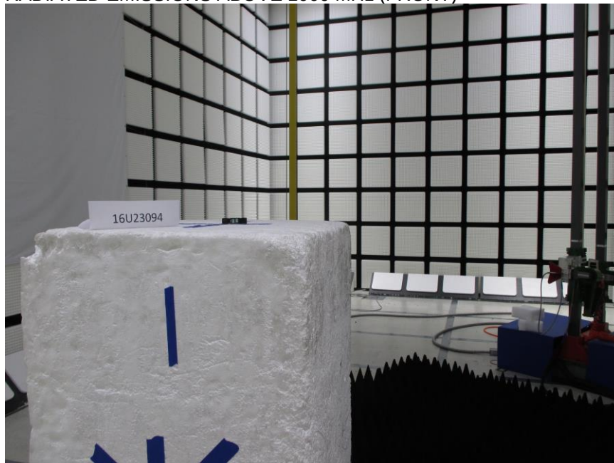
RADIATED EMISSIONS ABOVE 1000 MHz (FRONT)
