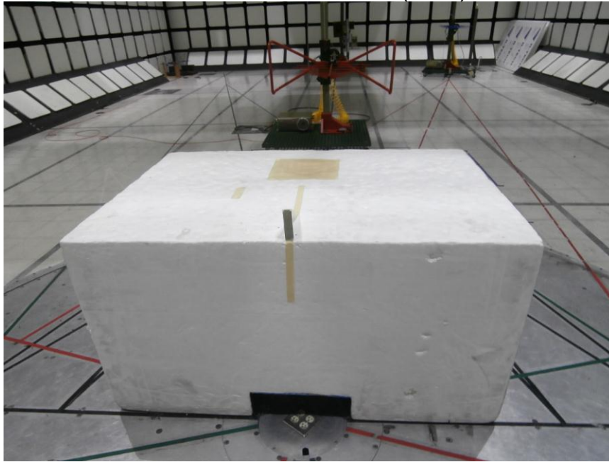
RADIATED EMISSIONS BELOW 1GHz30MHz (BACK)
