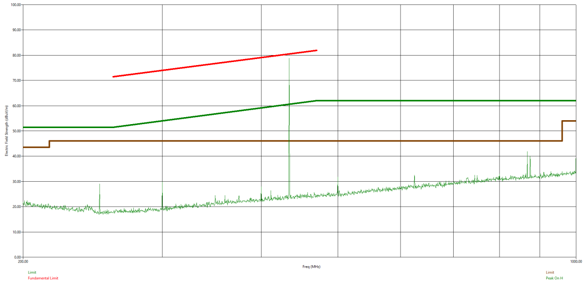
Figure 5: RE graph using peak detector on Horizontal polarization from 200MHz to 1GHz
