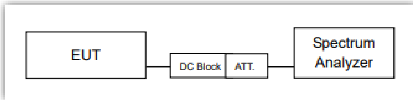
Figure 17: Typical test setup for Transmitter Time
