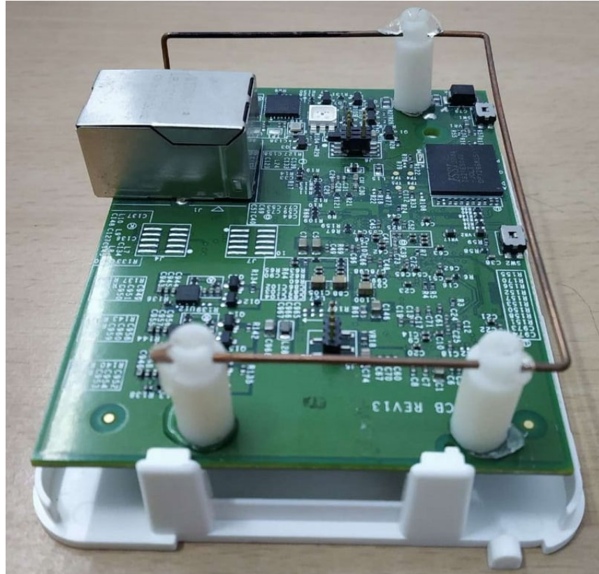
Figure 18 Photograph of Monopole Copper-Clad antenna installed in the product
