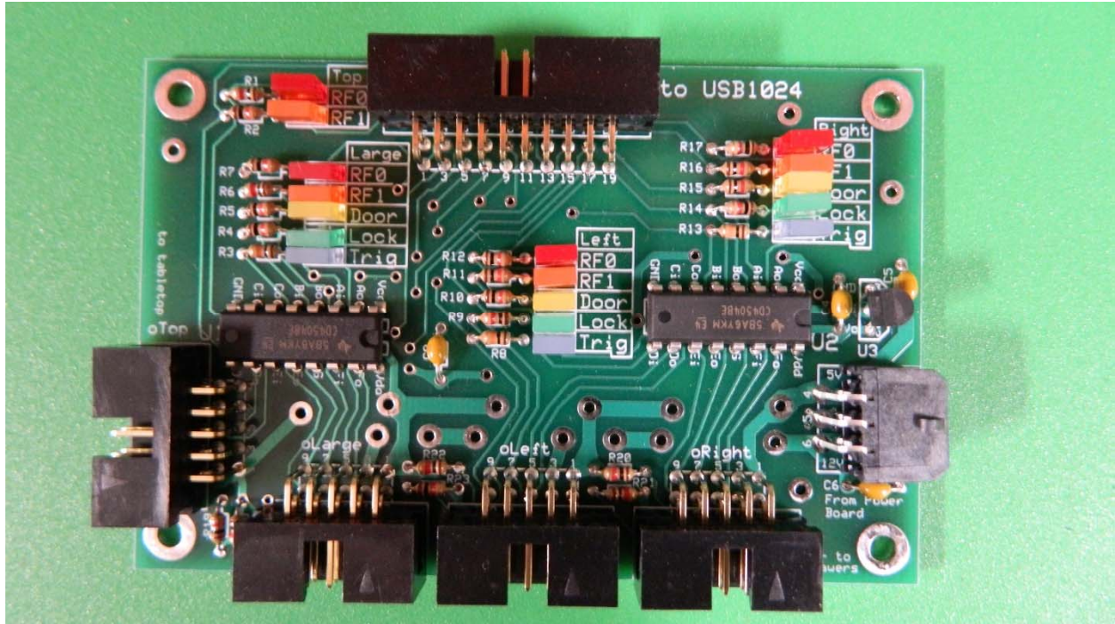
MEPS Logic/Controller PCBA (top-side)
