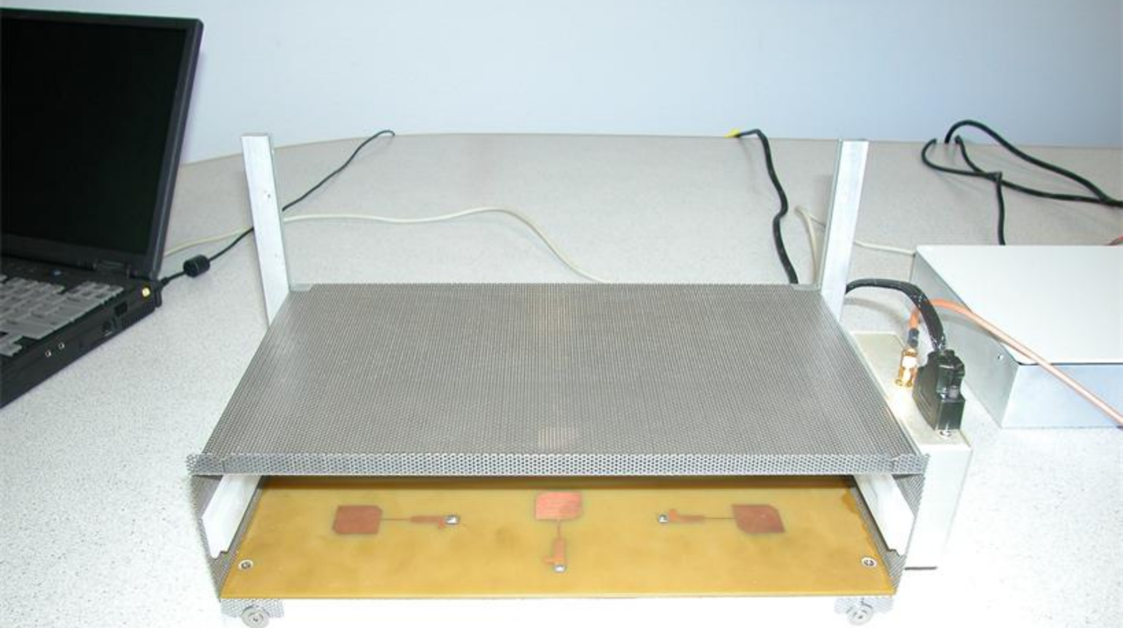
Six Antenna Array PCB Module Front View
