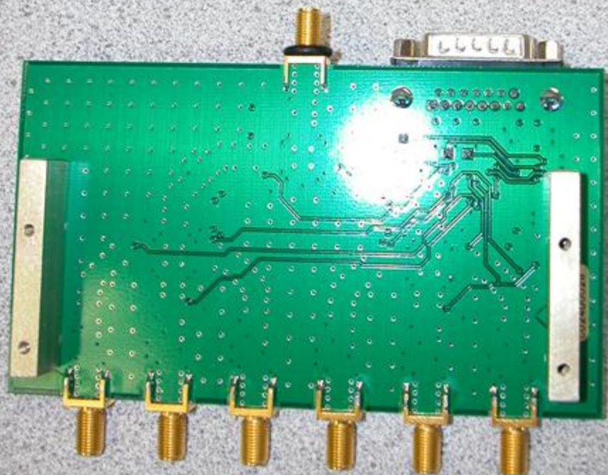
RF Switch PCB Back Side Out of Enclosure
