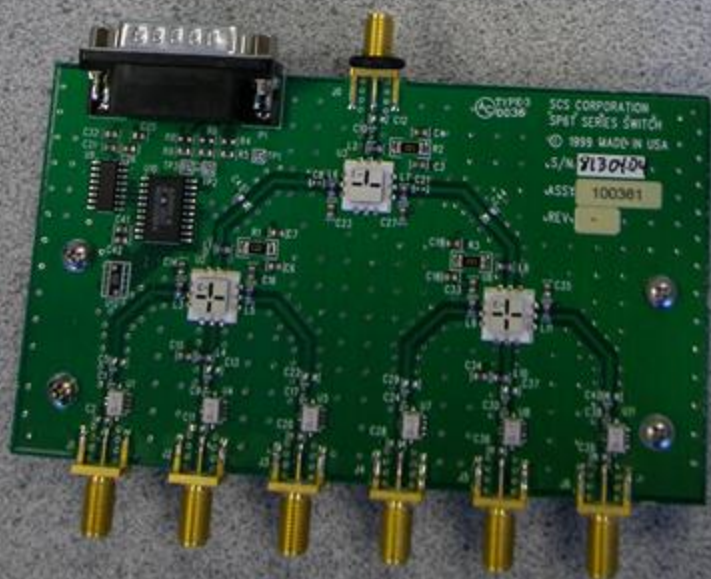
Open Assembly PCB Top
