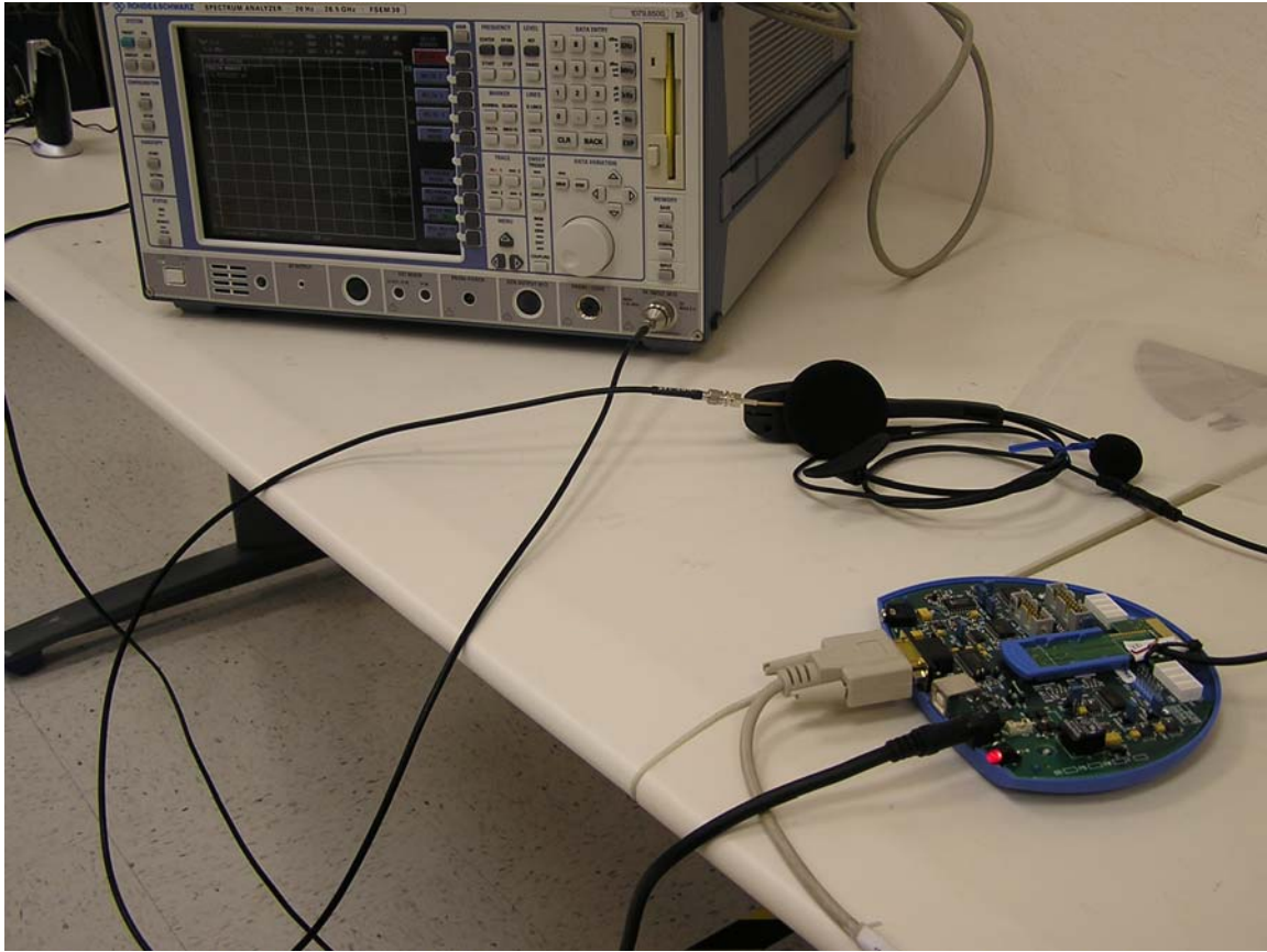
Test set up – Conducted measurements (EUT hooked to Cassira Kit from CSR for setting test mode)
