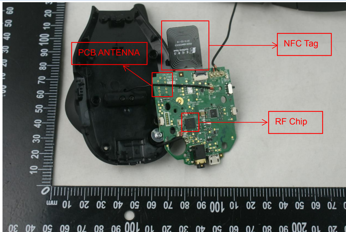
MAIN BOARD 1 FRONT VIEW
