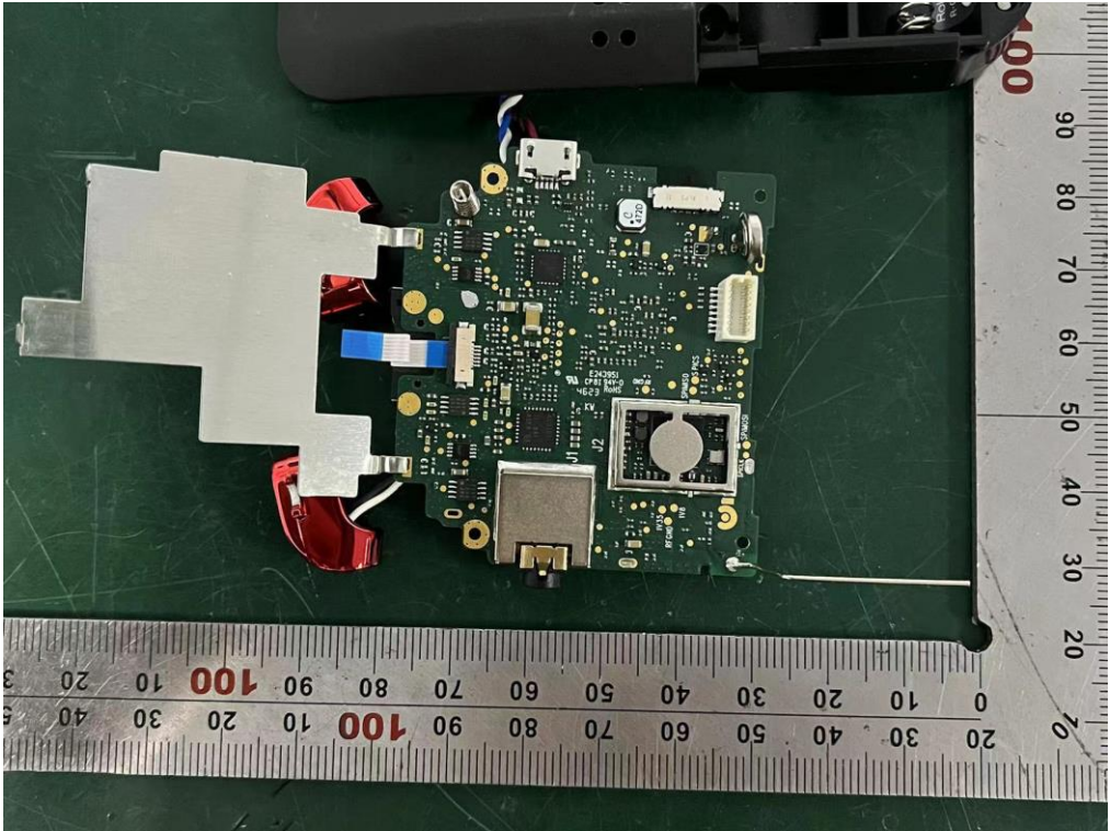
Internal Photos M/N: R-07
