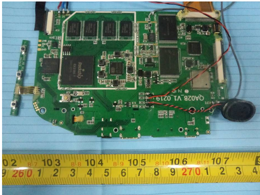
EUT (Pad) – Main Board Top Shielding off View
