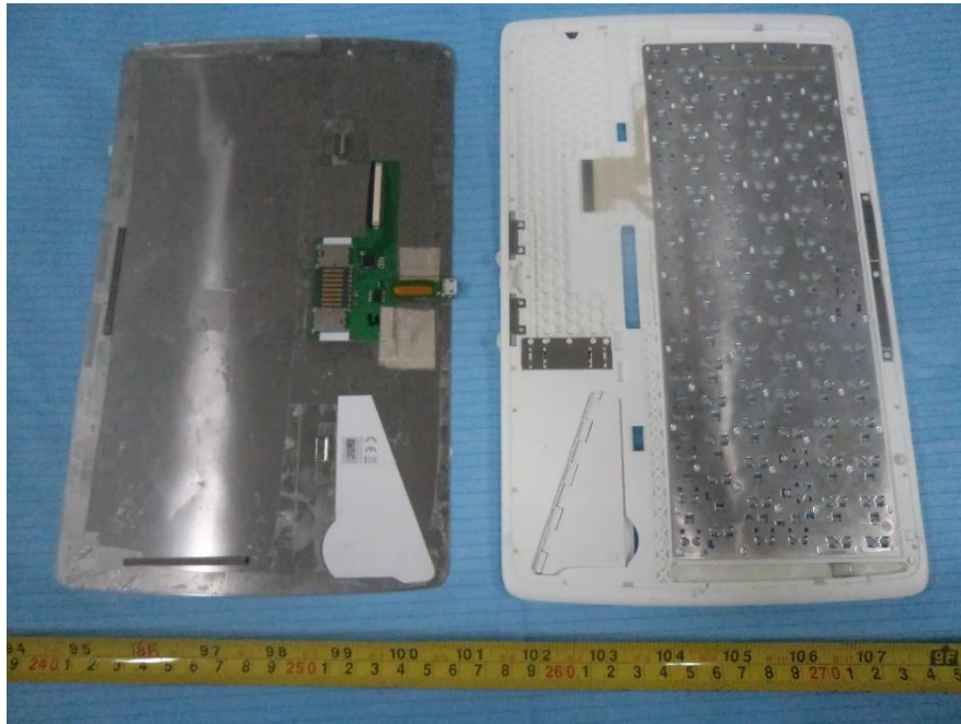
EUT (Keyboard) – Cover off View
