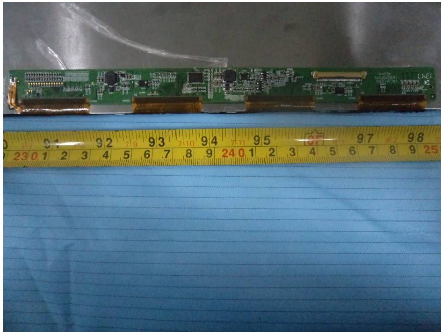
EUT (Pad) – Sub-board Top View
