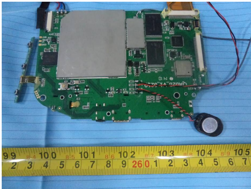
EUT (Pad) – Main Board Top View
