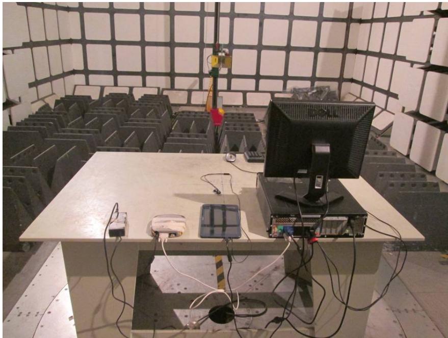
Radiated Emissions – Rear View (Above 1 GHz) (Downloading Mode)
