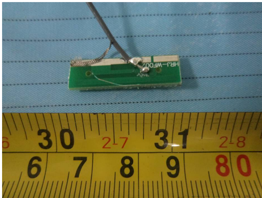
EUT – Bluetooth & Wi-Fi Antenna View
