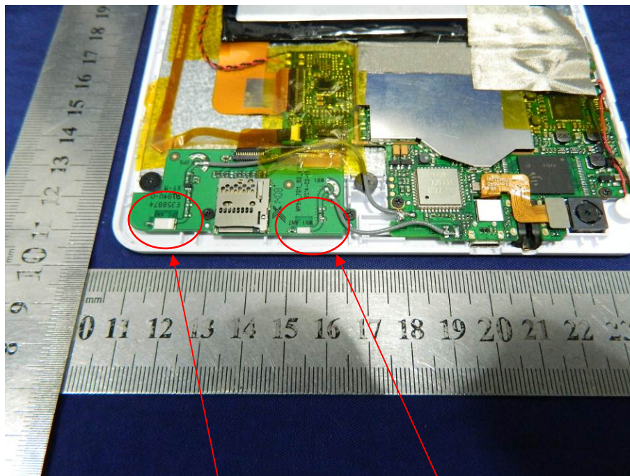
Wifi & Bluetooth Antenna
