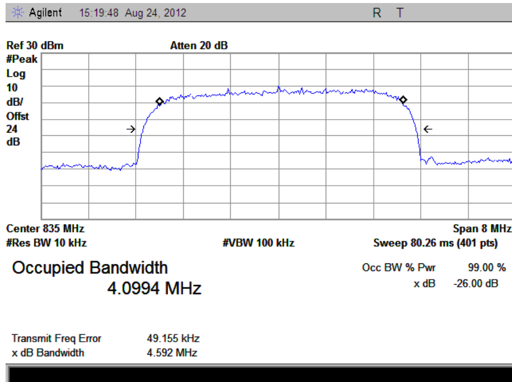
(Plot C: HSDPA 850MHz Channel = 4175)
