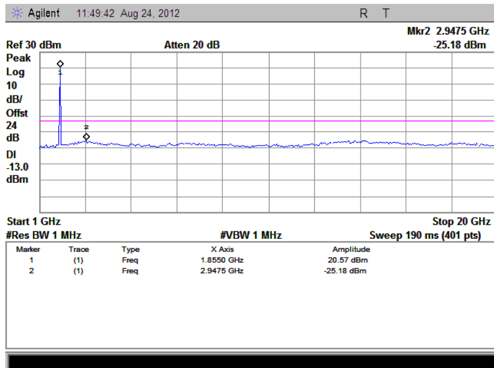
(Plot B1.1: WCDMA1900MHz Channel = 9262, 1GHz to 20GHz)
