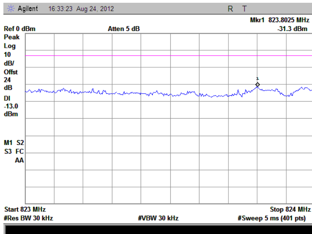
(Plot I: HSUPA 850 Channel = 4132)
