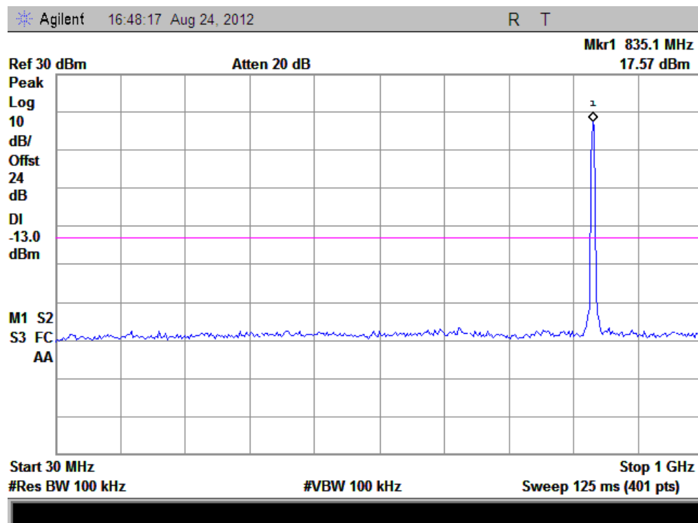
(Plot E 2: HSUPA 850MHz Channel = 4175, 30MHz to 1GHz)
