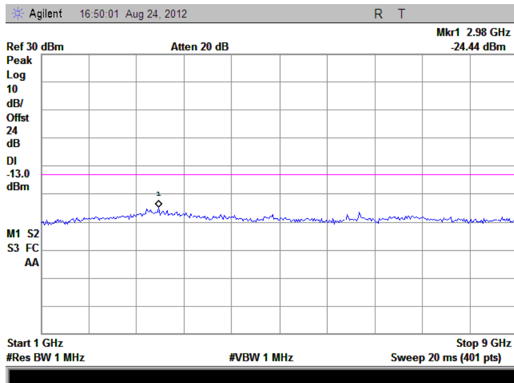
(Plot E3.1: HSUPA850MHz Channel = 4233, 1GHz to 9GHz)
