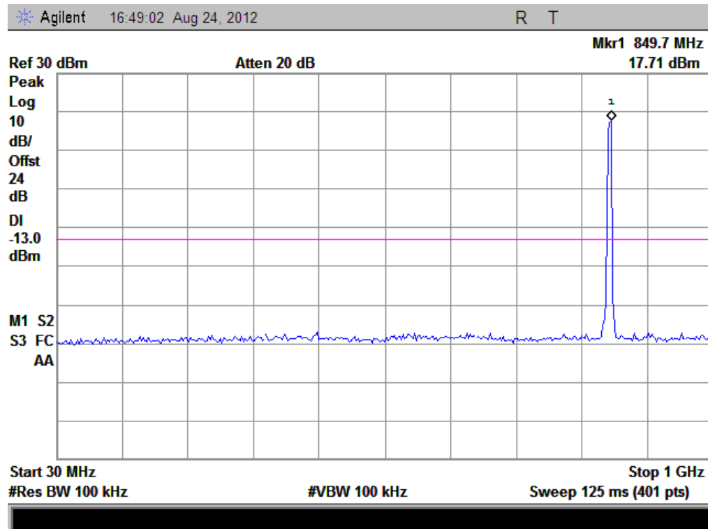
(Plot E 3: HSUPA850MHz Channel = 4233, 30MHz to 1GHz)
