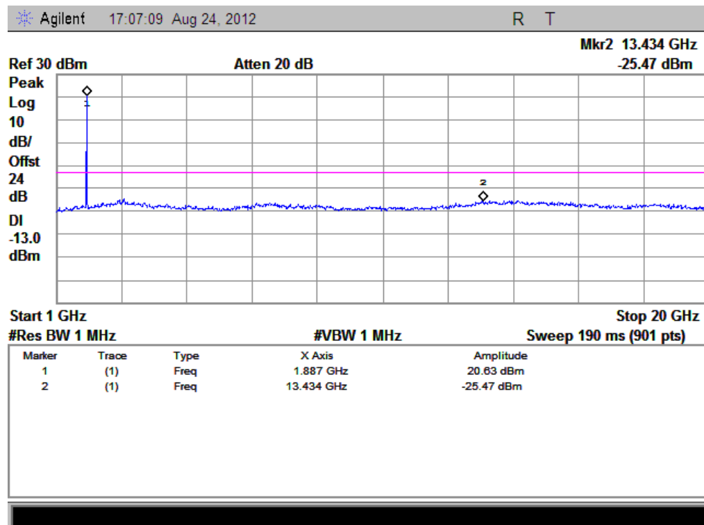
(Plot F2.1: HSUPA1900MHz Channel = 9400, 1GHz to 20GHz)
