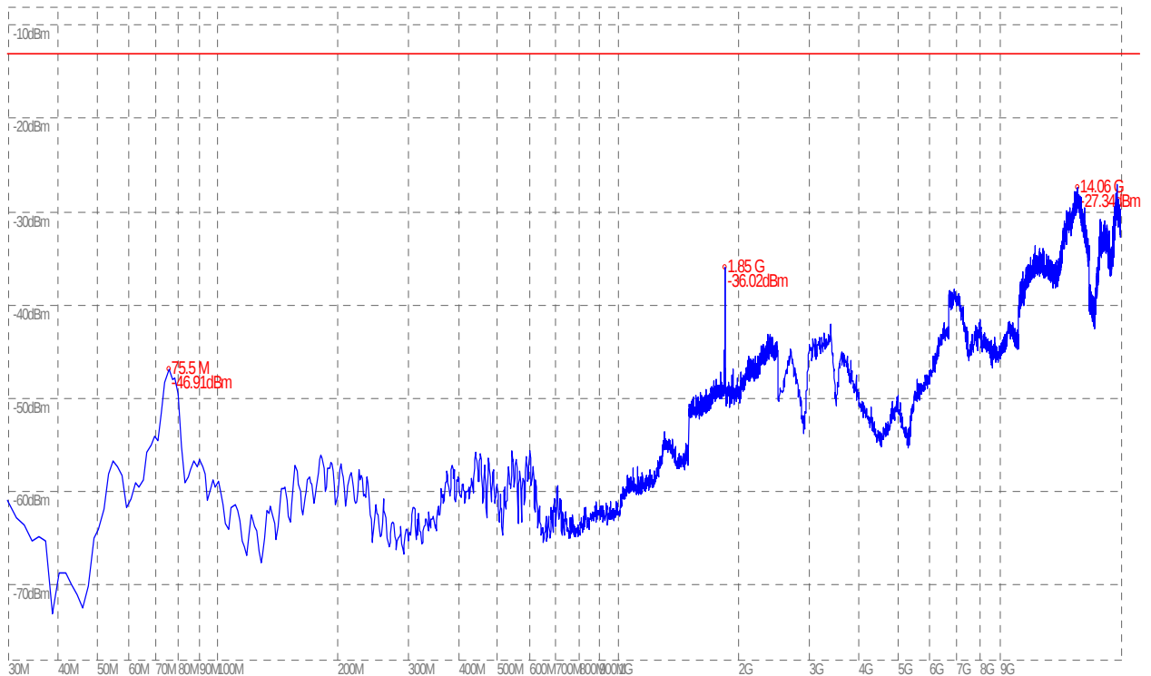
(Plot F.5: WCDMA 1900MHz Channel = 9538, Test Antenna Horizontal)
