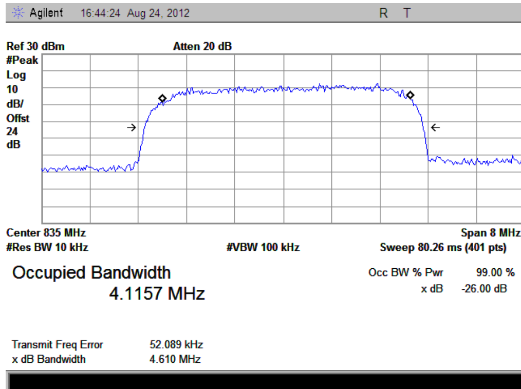
(Plot E: HSUPA 850MHz Channel = 4175)
