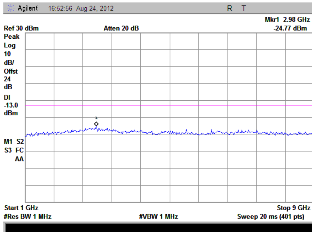
(Plot E1.1: HSUPA 850MHz Channel = 4132, 1GHz to 9GHz)
