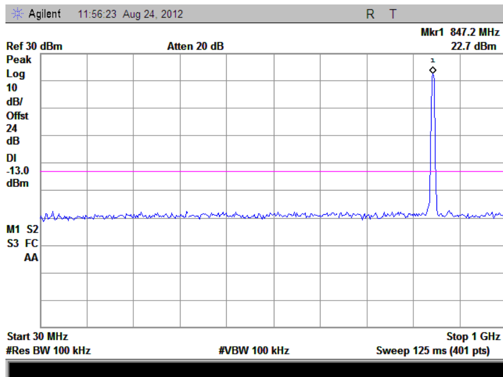
(Plot A3: WCDMA850MHz Channel = 4233, 30MHz to 1GHz)
