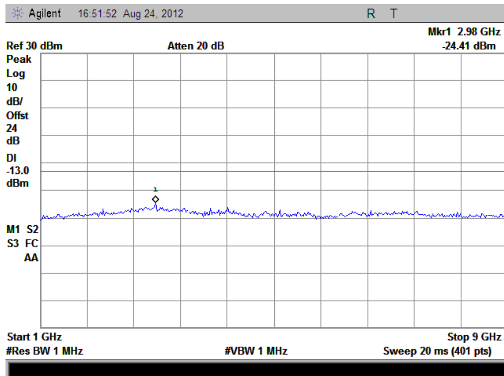
(Plot E2.1: HSUPA 850MHz Channel = 4175, 1GHz to 9GHz)
