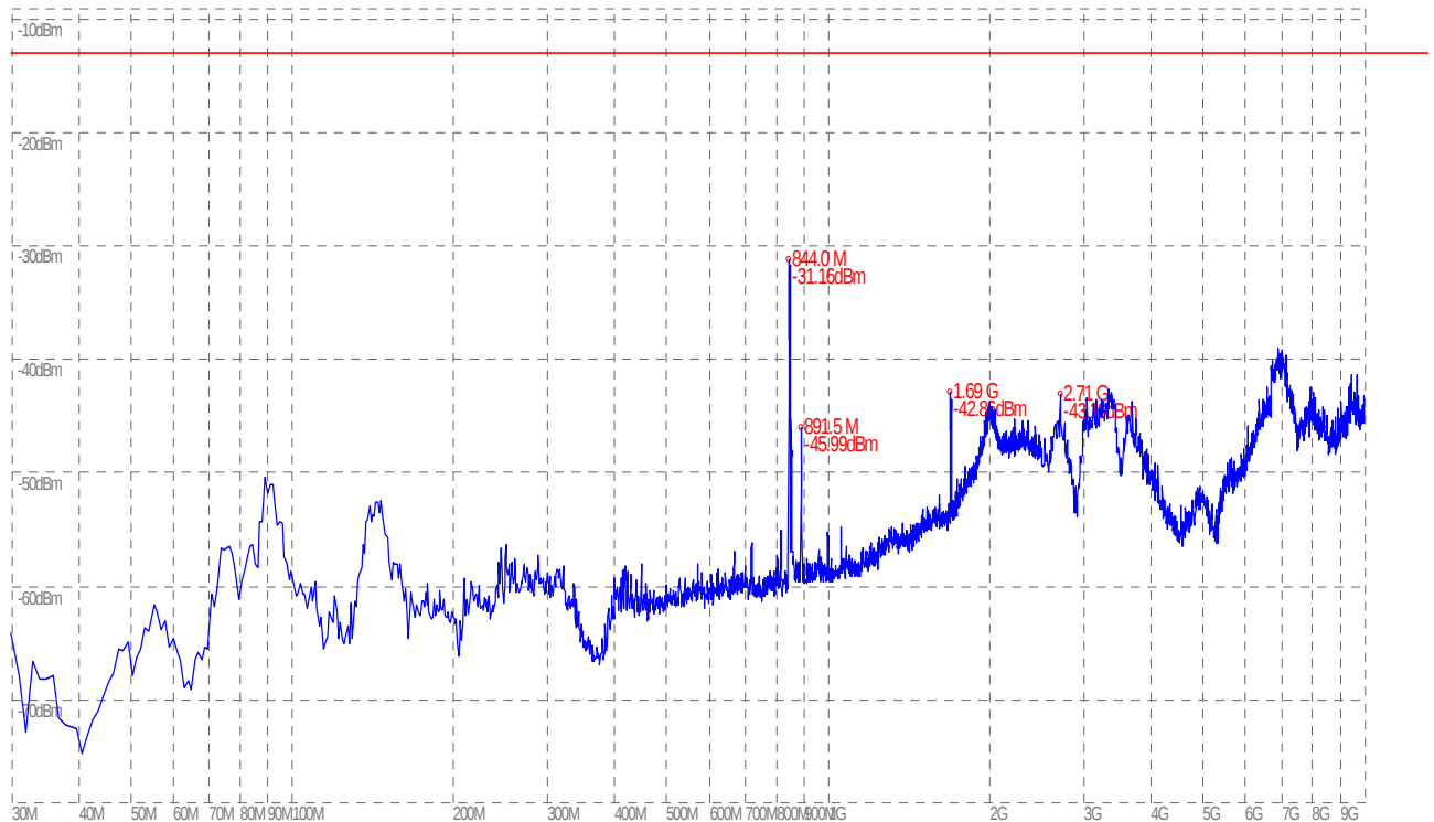
(Plot I.5: HSUPA 850MHz Channel = 4233, Test Antenna Horizontal)
