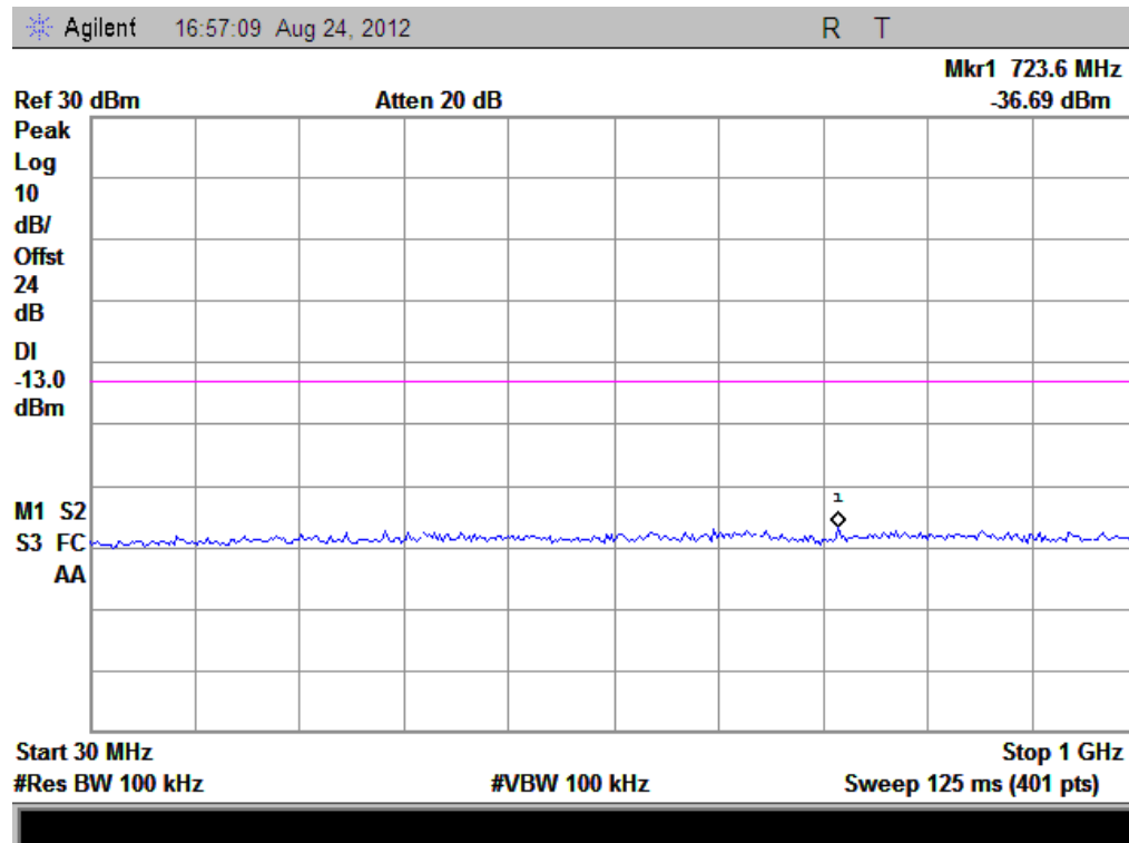
(Plot F 2: HSUPA1900MHz Channel = 9400, 30MHz to 1GHz)
