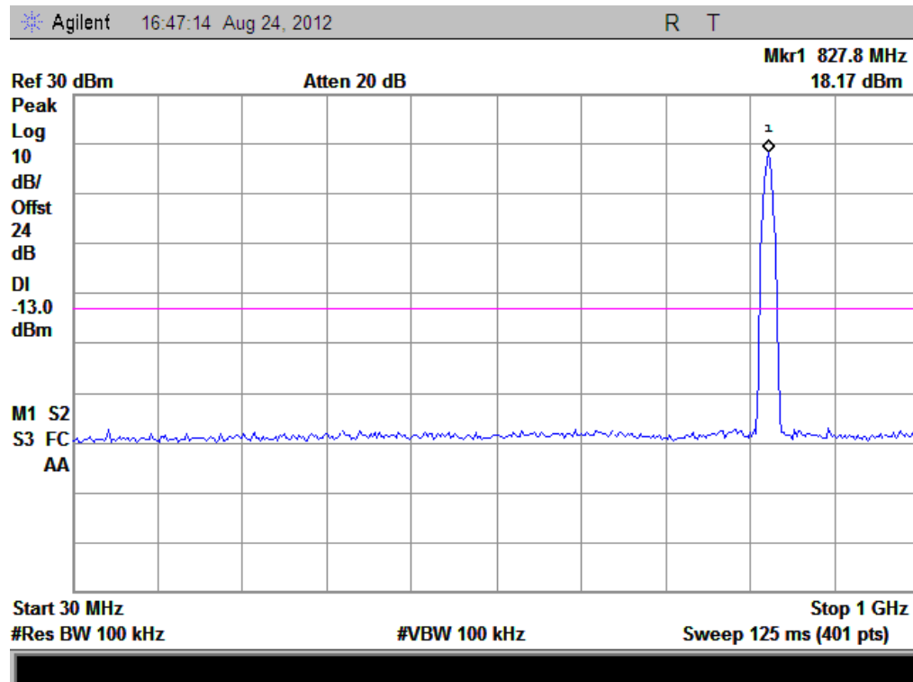
(Plot E 1: HSUPA 850MHz Channel = 4132, 30MHz to 1GHz)
