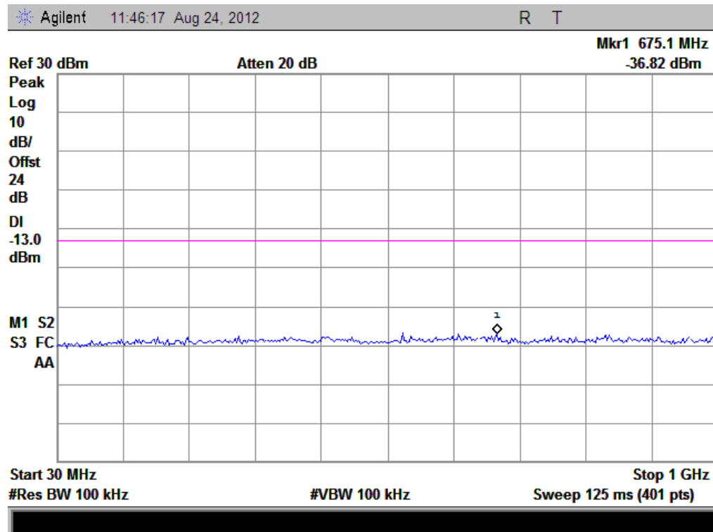
(Plot B2: WCDMA1900MHz Channel = 9400, 30MHz to 1GHz)
