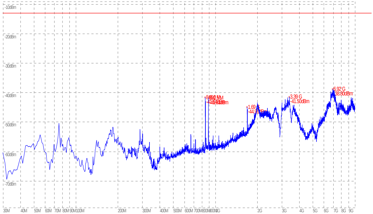
(Plot I.6: HSUPA 850MHz Channel = 4233, Test Antenna Vertical)
