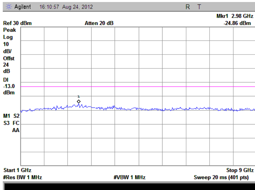
(Plot C3.1: HSDPA850MHz Channel = 4233, 1GHz to 9GHz)
