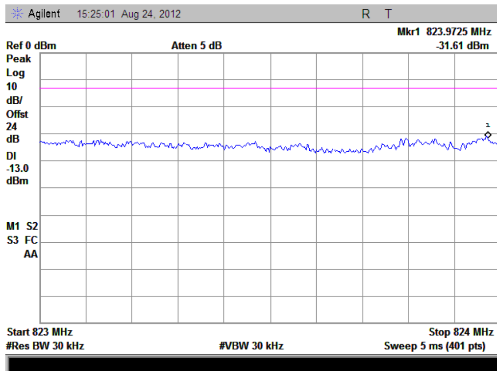
(Plot E: HSDPA 850 Channel = 4132)
