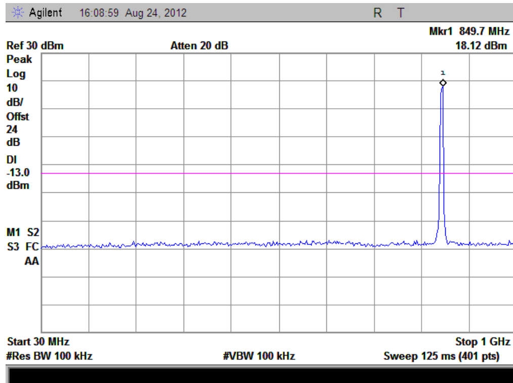
(Plot C3: HSDPA850MHz Channel = 4233, 30MHz to 1GHz)
