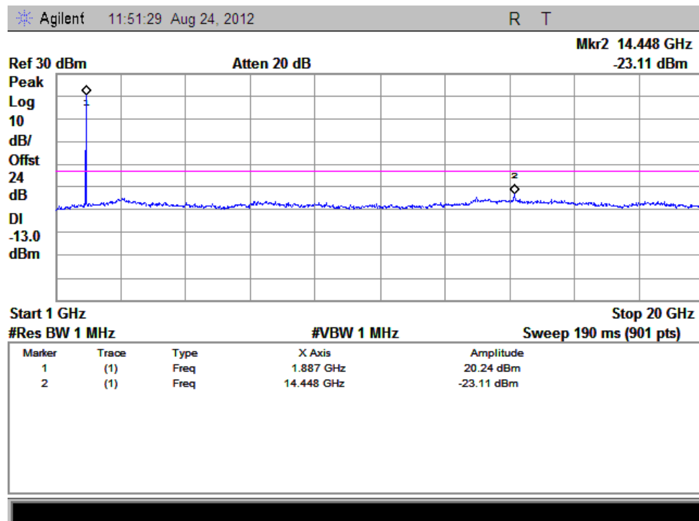
(Plot B2.1: WCDMA1900MHz Channel = 9400, 1GHz to 20GHz)
