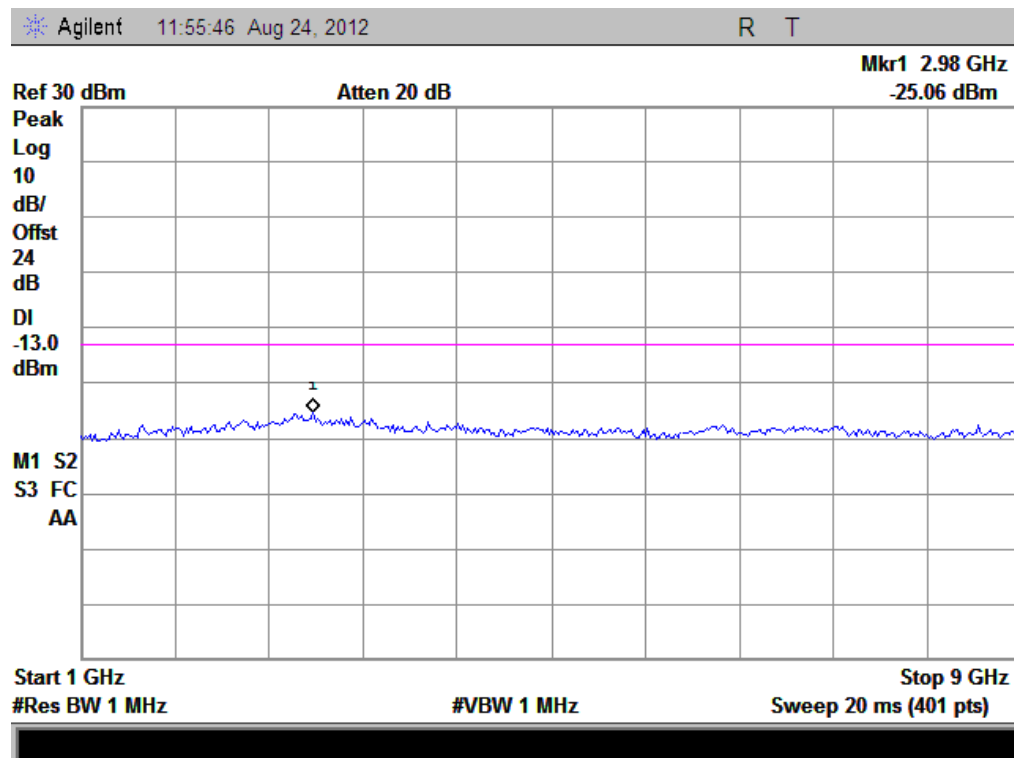
(Plot A3.1: WCDMA850MHz Channel = 4233, 1GHz to 9GHz)
