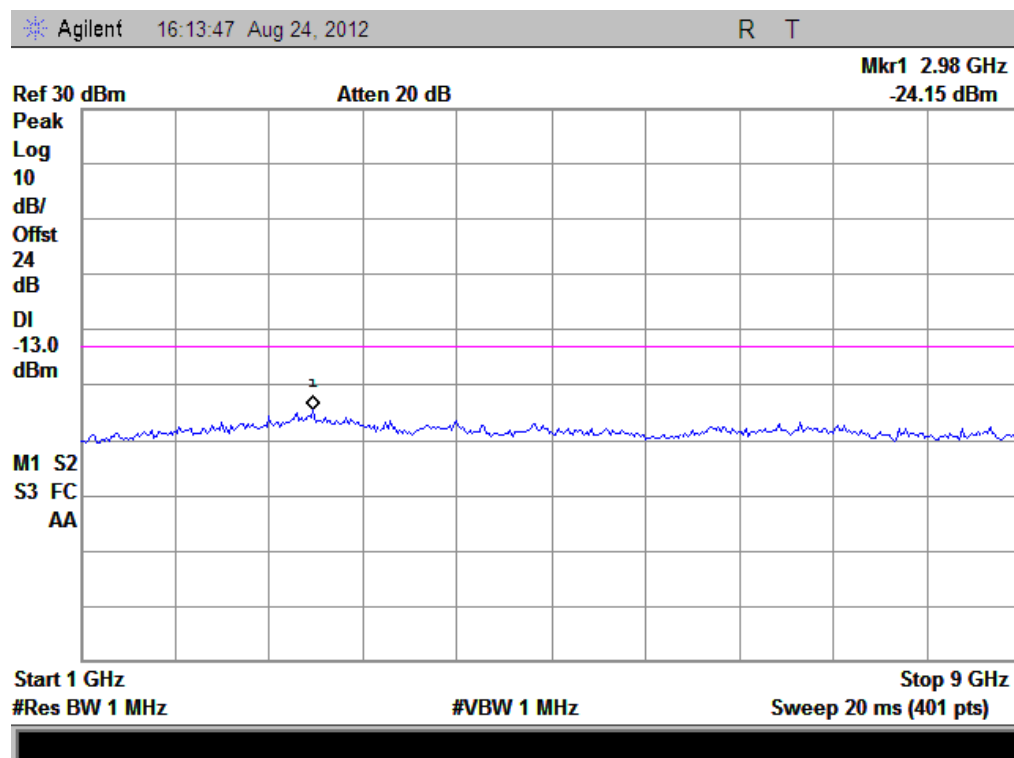
(Plot C1.1: HSDPA 850MHz Channel = 4132, 1GHz to 9GHz)
