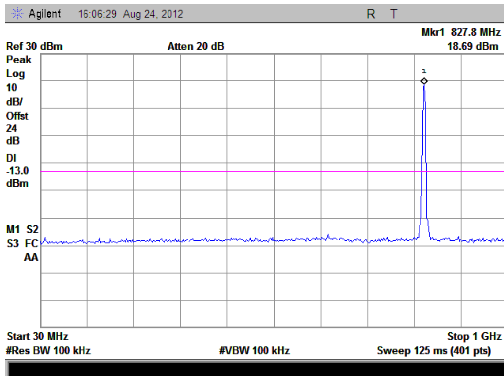
(Plot C1: HSDPA 850MHz Channel = 4132, 30MHz to 1GHz)
