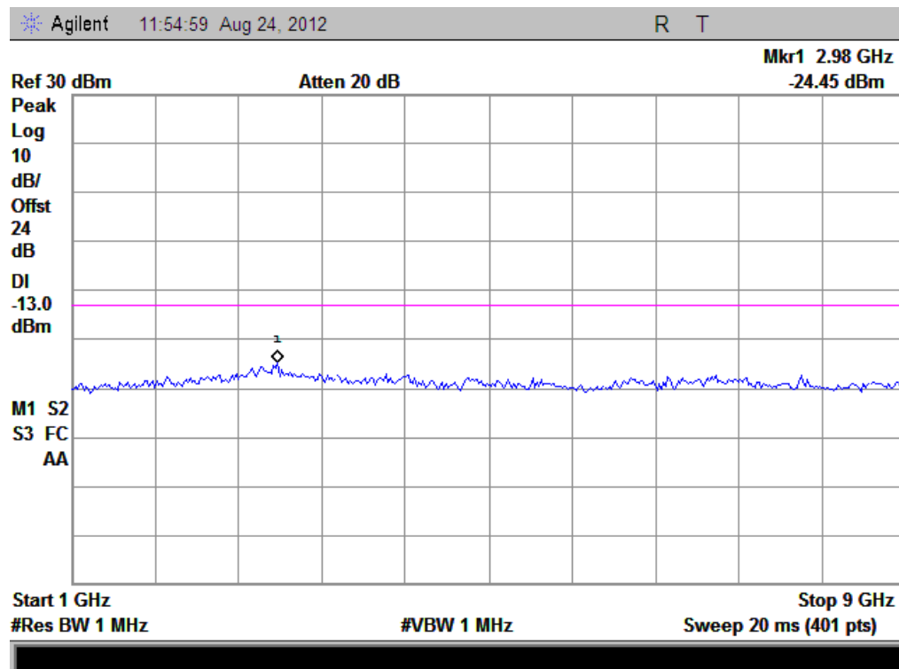
(Plot A2.1: WCDMA850MHz Channel = 4175, 1GHz to 9GHz)
