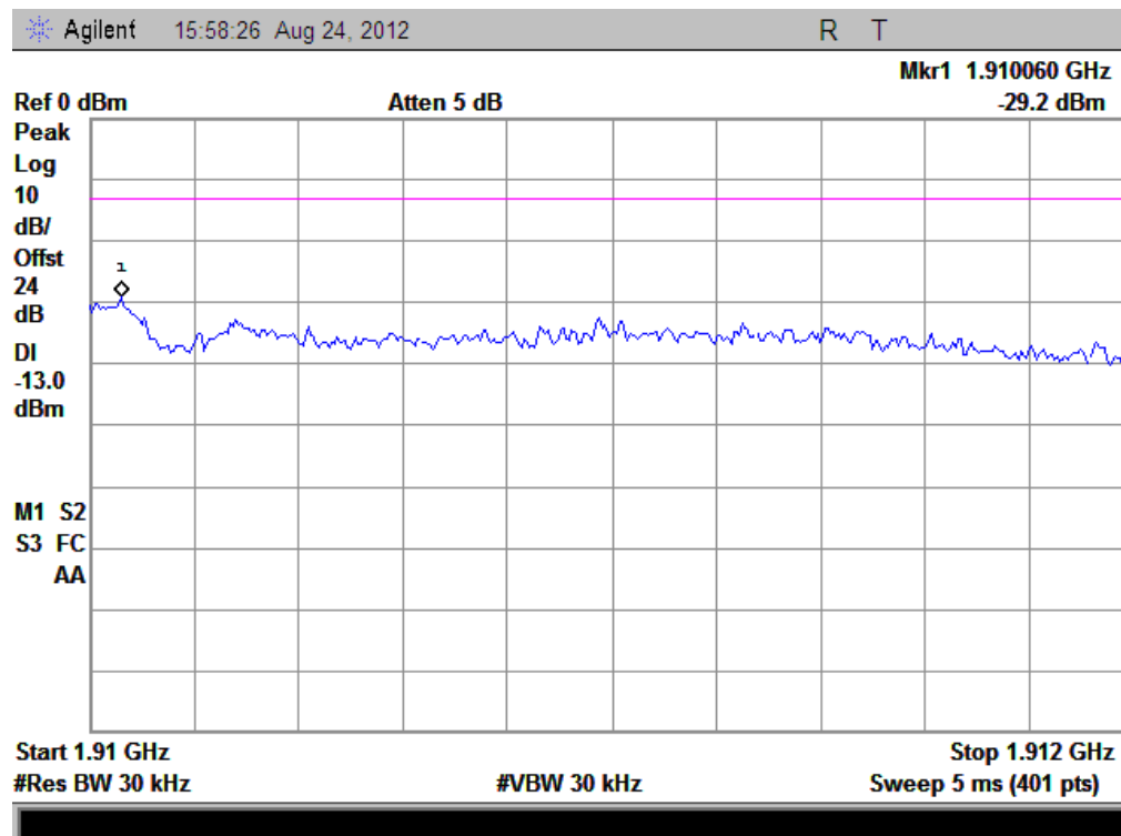
(Plot L: HSUPA 1900 Channel = 9538)
