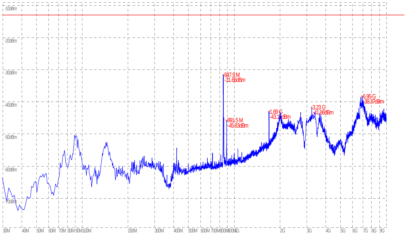
(Plot I.1: HSUPA 850MHz Channel = 4132, Test Antenna Horizontal)
