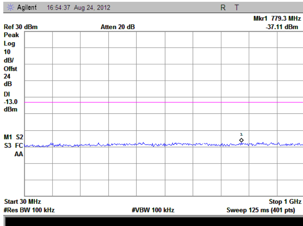
(Plot F 1: HSUPA1900MHz Channel = 9262, 30MHz to 1GHz)
