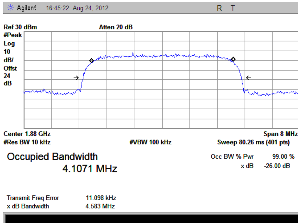
(Plot F: HSUPA1900MHz Channel = 9400)
