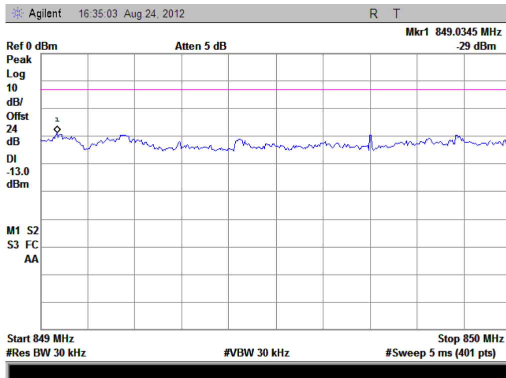
(Plot J: HSUPA850 Channel = 4233)
