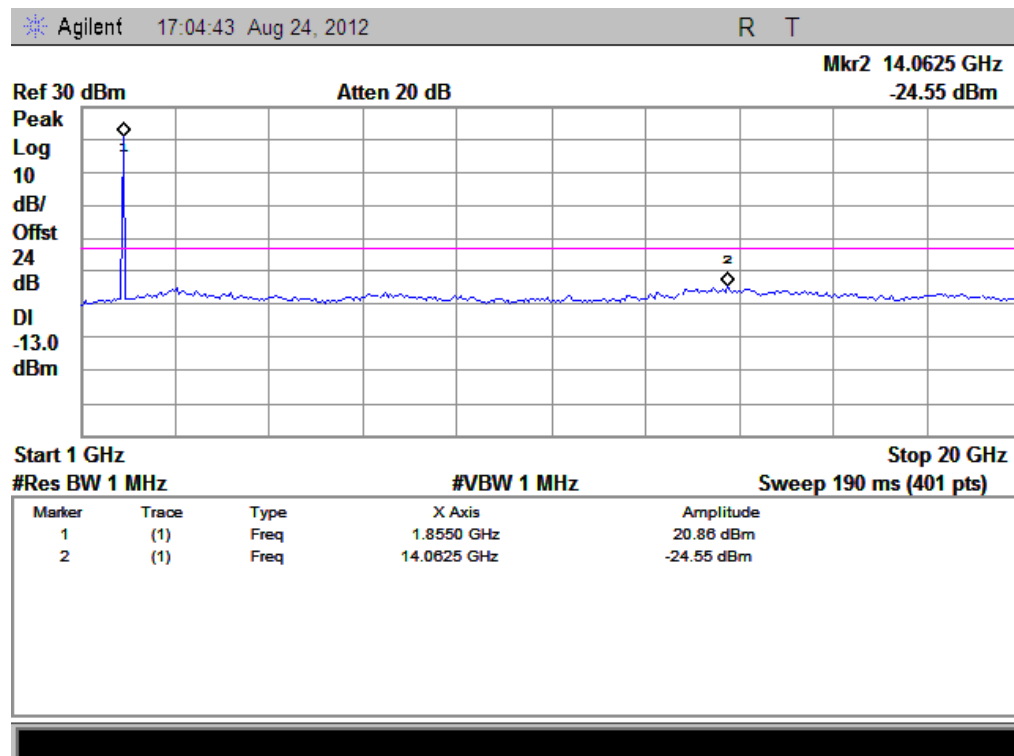
(Plot F1.1: HSUPA1900MHz Channel = 9262, 1GHz to 20GHz)
