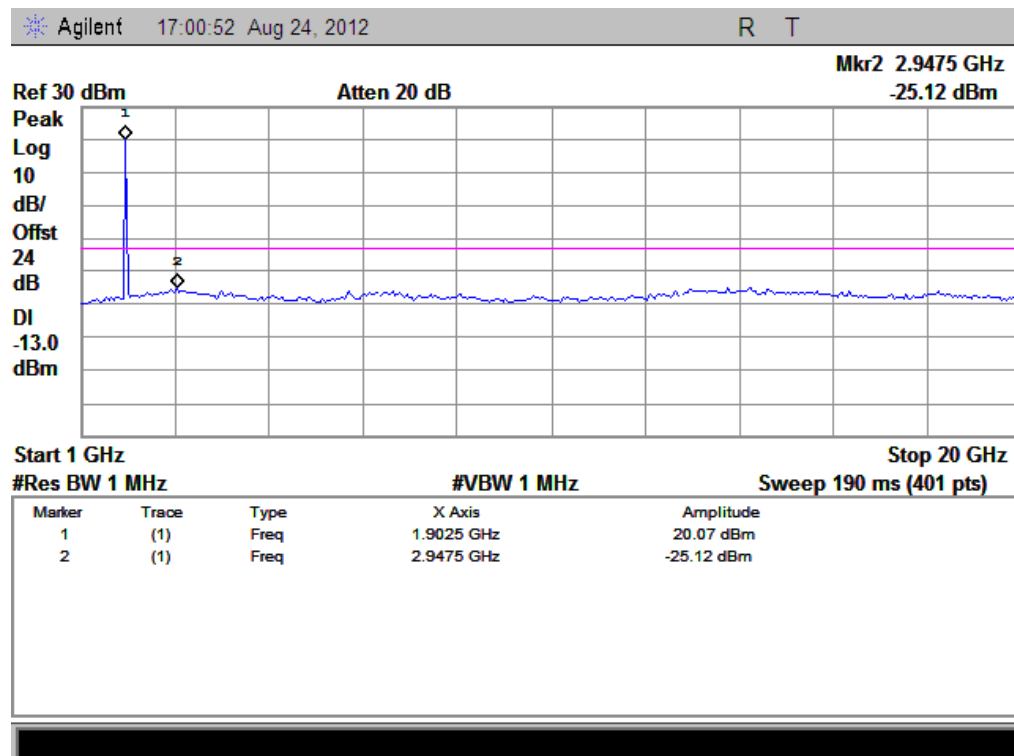
(Plot F3.1: HSUPA1900MHz Channel = 9538 1GHz to 20GHz)
