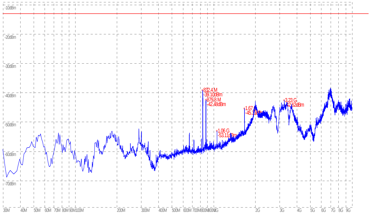
(Plot G.6: HSDPA 850MHz Channel = 4233, Test Antenna Vertical)
