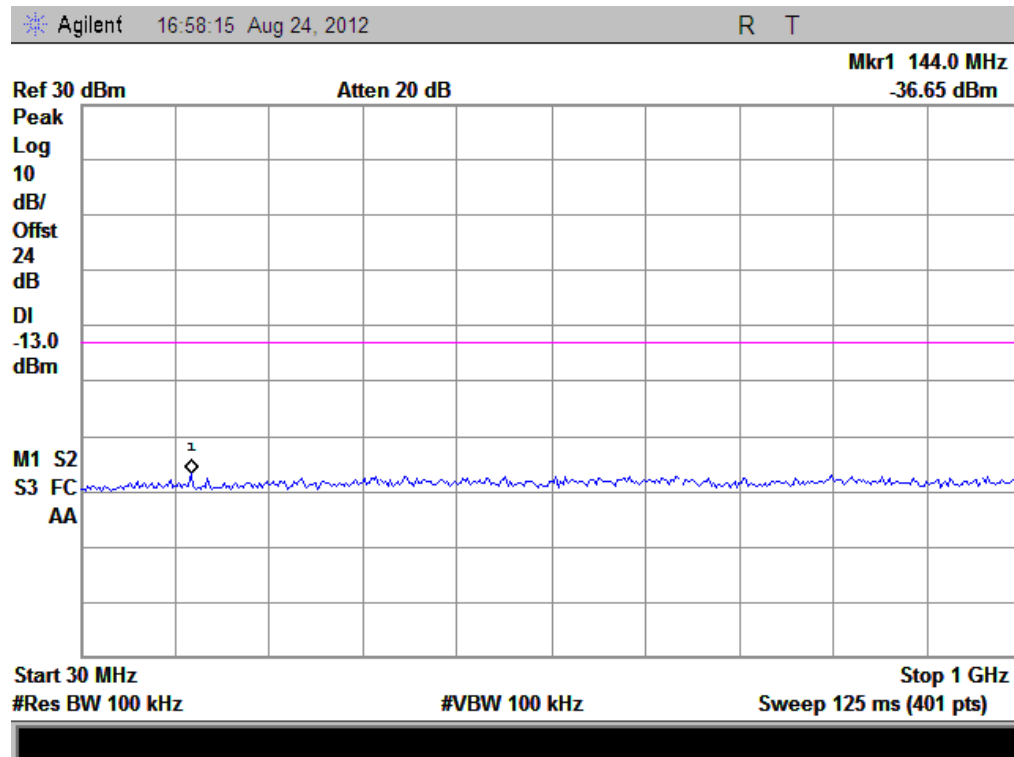
(Plot F 3: HSUPA1900MHz Channel = 9538, 30MHz to 1GHz)
