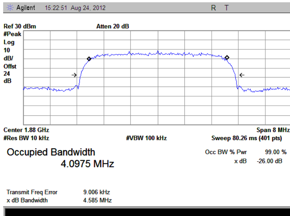
(Plot D: HSDPA1900MHz Channel = 9400)
