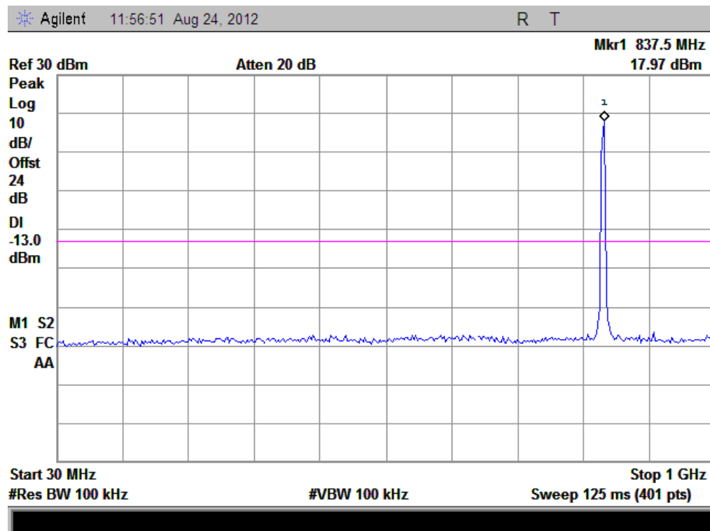
(Plot A2: WCDMA850MHz Channel = 4175, 30MHz to 1GHz)
