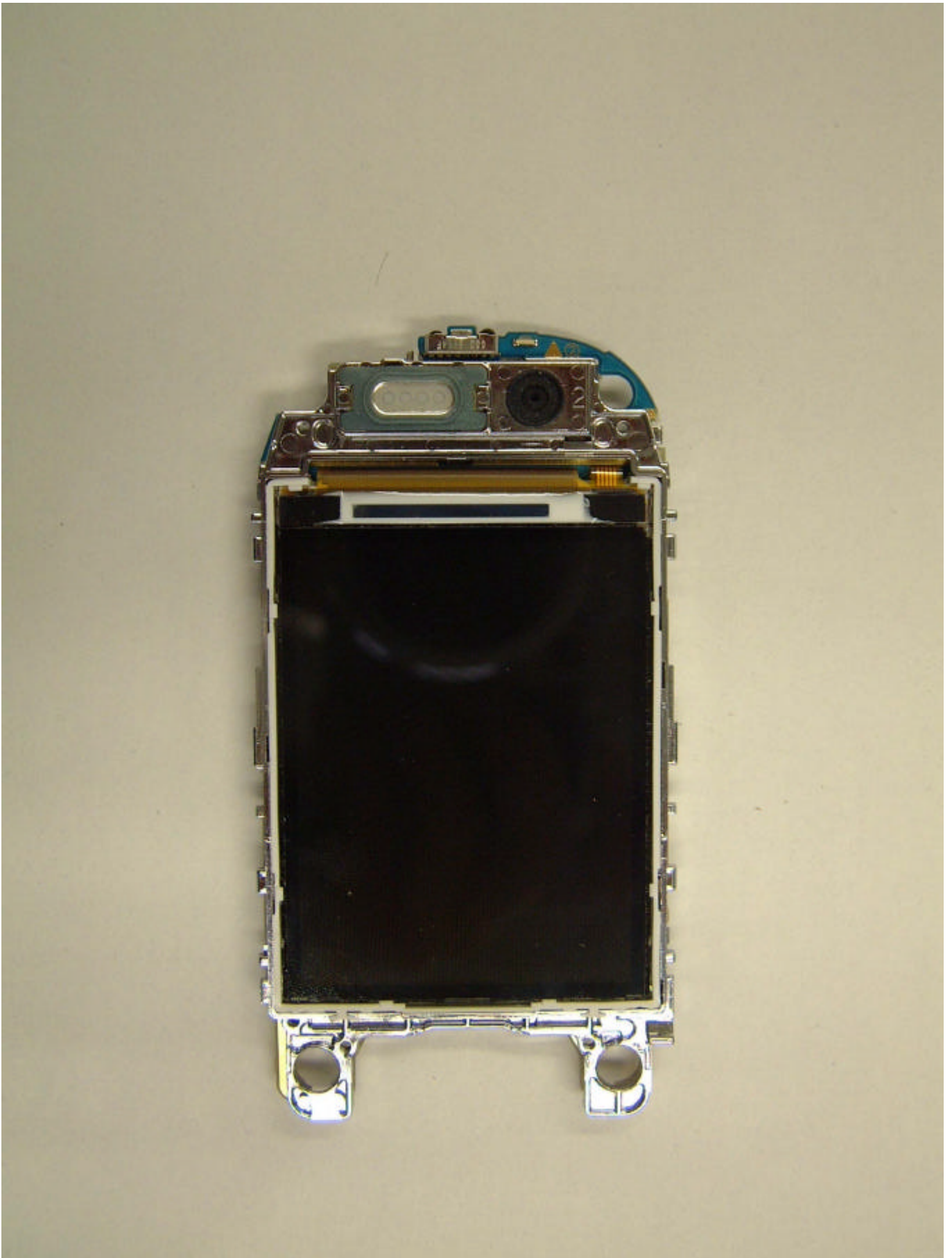
Upper PCB within Main LCD
