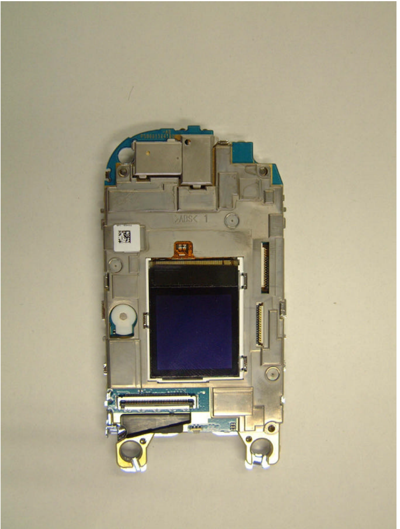
Upper PCB within Sub LCD and Shield Case
