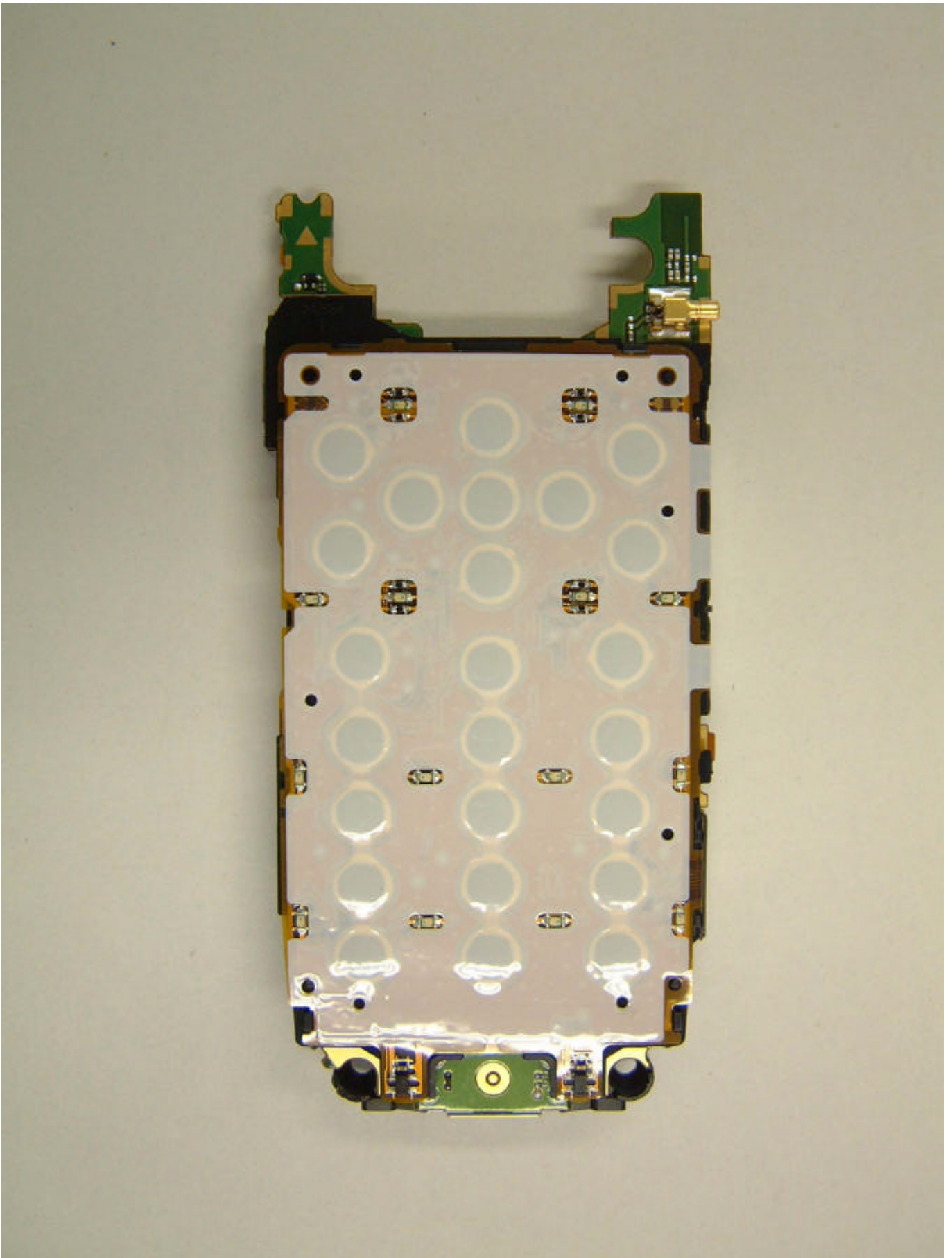
Lower PCB within key Assembly article
