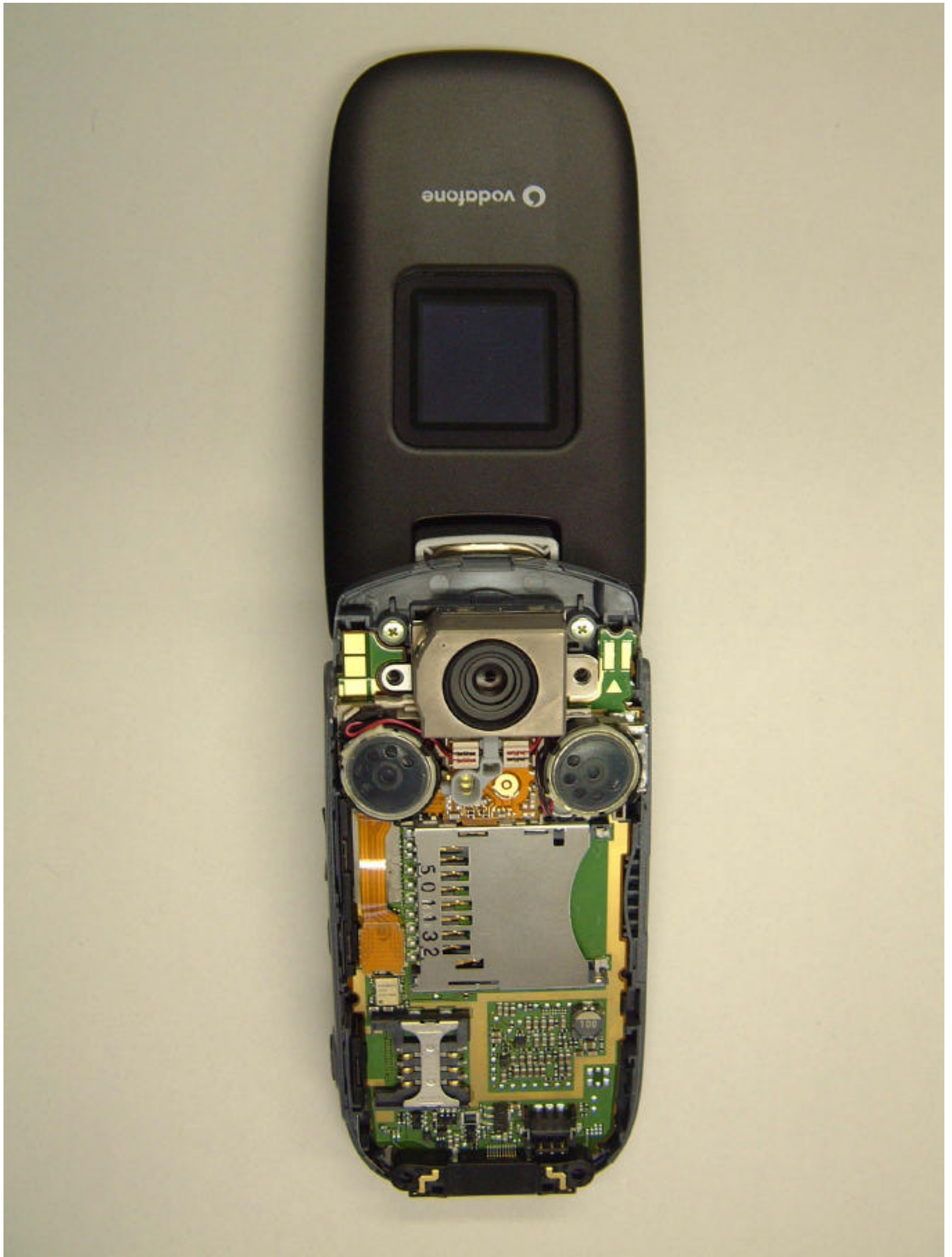
Equipment within Upper PCB
