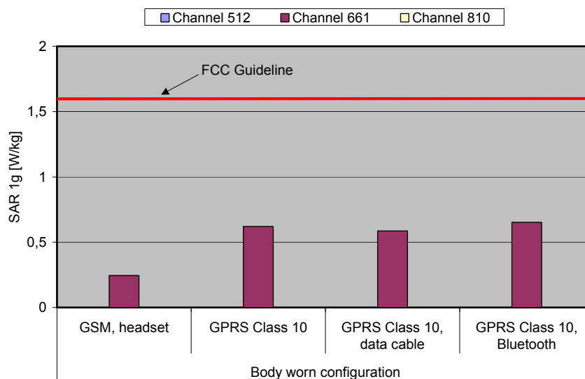
Fig. 9: The measured SAR values in body-worn configuration for the Toshiba TS 921 for PCS 1900 in comparison to the FCC exposure limit.
