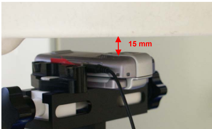
Fig. 21: Body worn configuration, GSM with headset, antenna towards the phantom.
