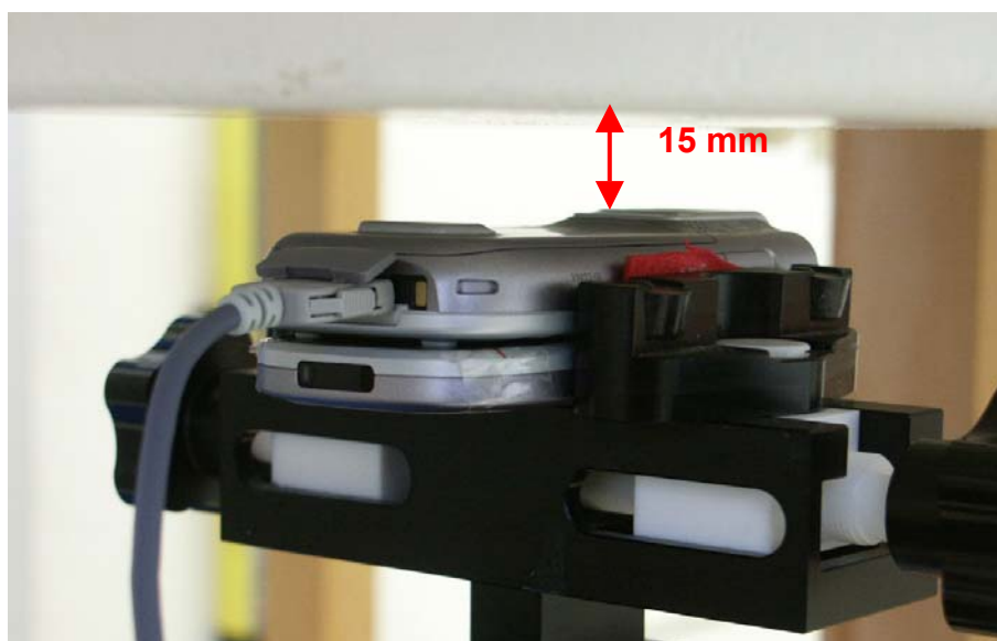
Fig. 23: Body worn configuration, GPRS(Class 10) with data cable, antenna towards the phantom.
