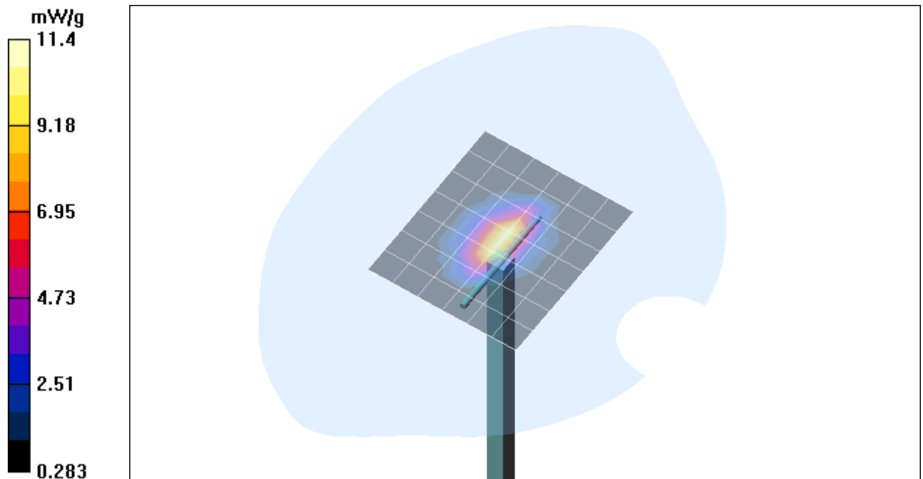
Fig. 11: Validation measurement 1900 MHz body (March 10, 2005), coarse grid. Ambient Temperature: 22.0° C, Liquid Temperature: 21.0° C.
