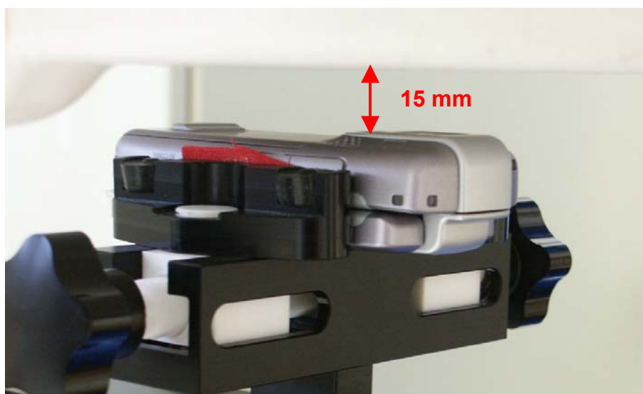
Fig. 22: Body worn configuration, GPRS (Class 10), antenna towards the phantom.
