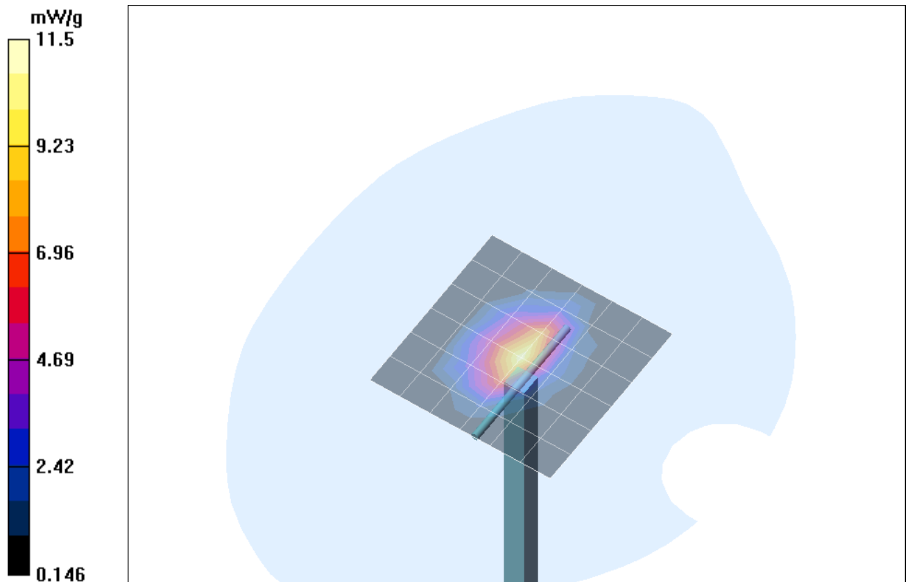
Fig. 10: Validation measurement 1900 MHz Head (March 09, 2005), coarse grid. Ambient Temperature: 22.0° C, Liquid Temperature: 21.0° C.
