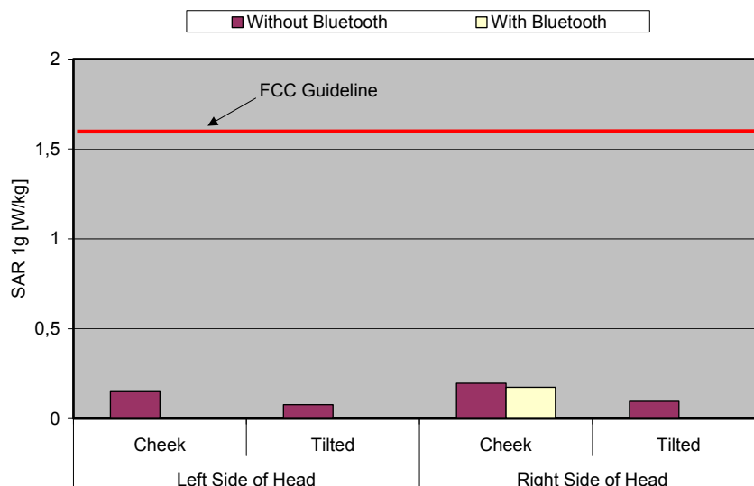
Fig. 8: The measured head phantom SAR values for the Toshiba TS 921 for PCS 1900 in comparison to the FCC exposure limit.
