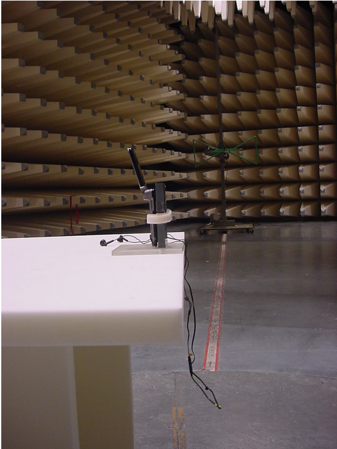
Photo 2 (Radiated Emissions):
