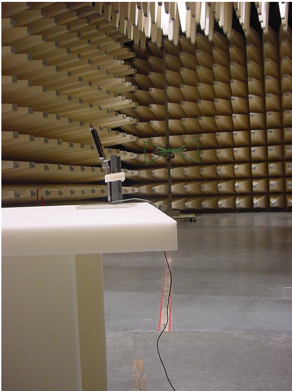
Photo 2 (Radiated Emissions):
