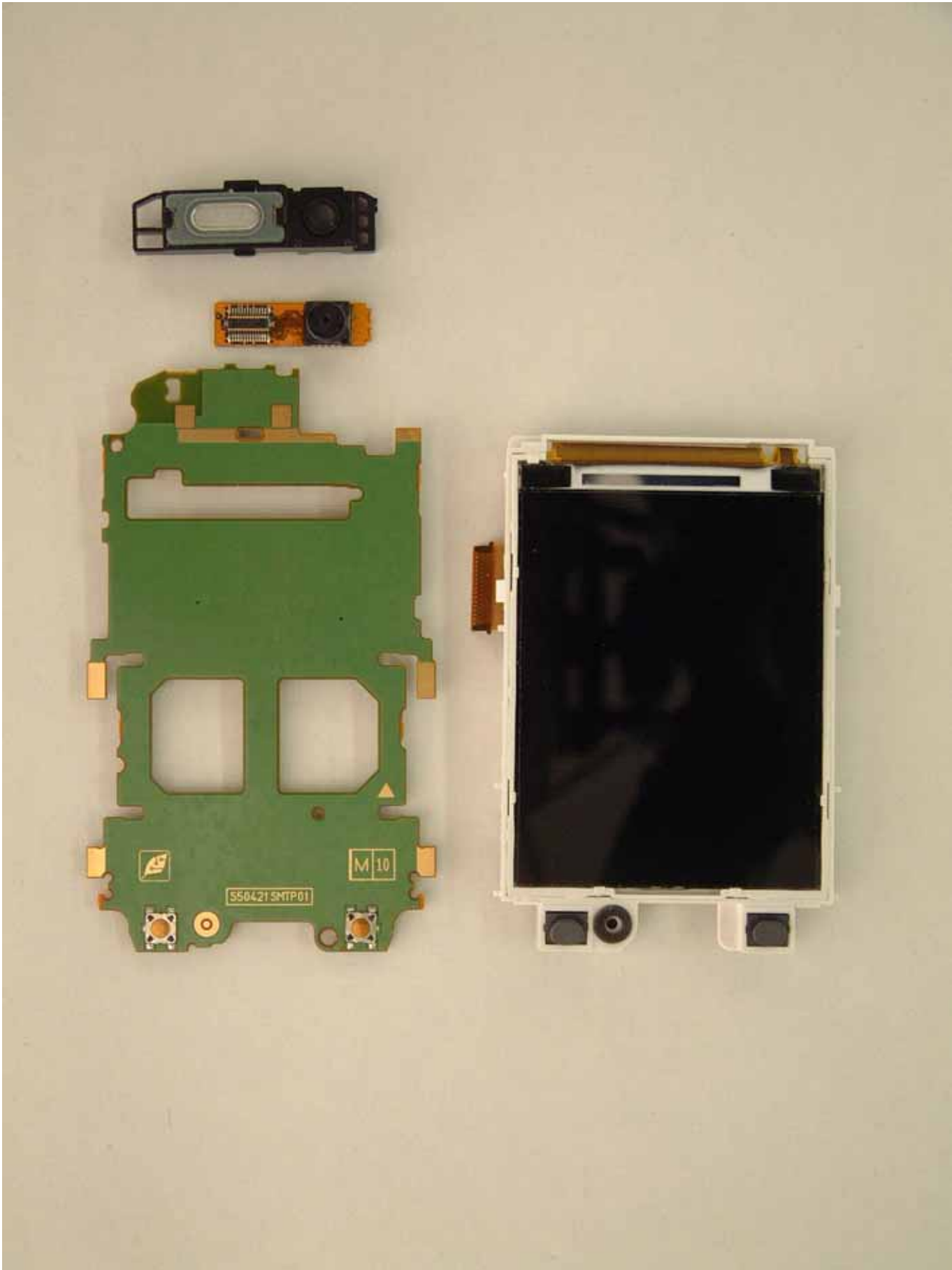
Upper PCB Assembly (Back side)
