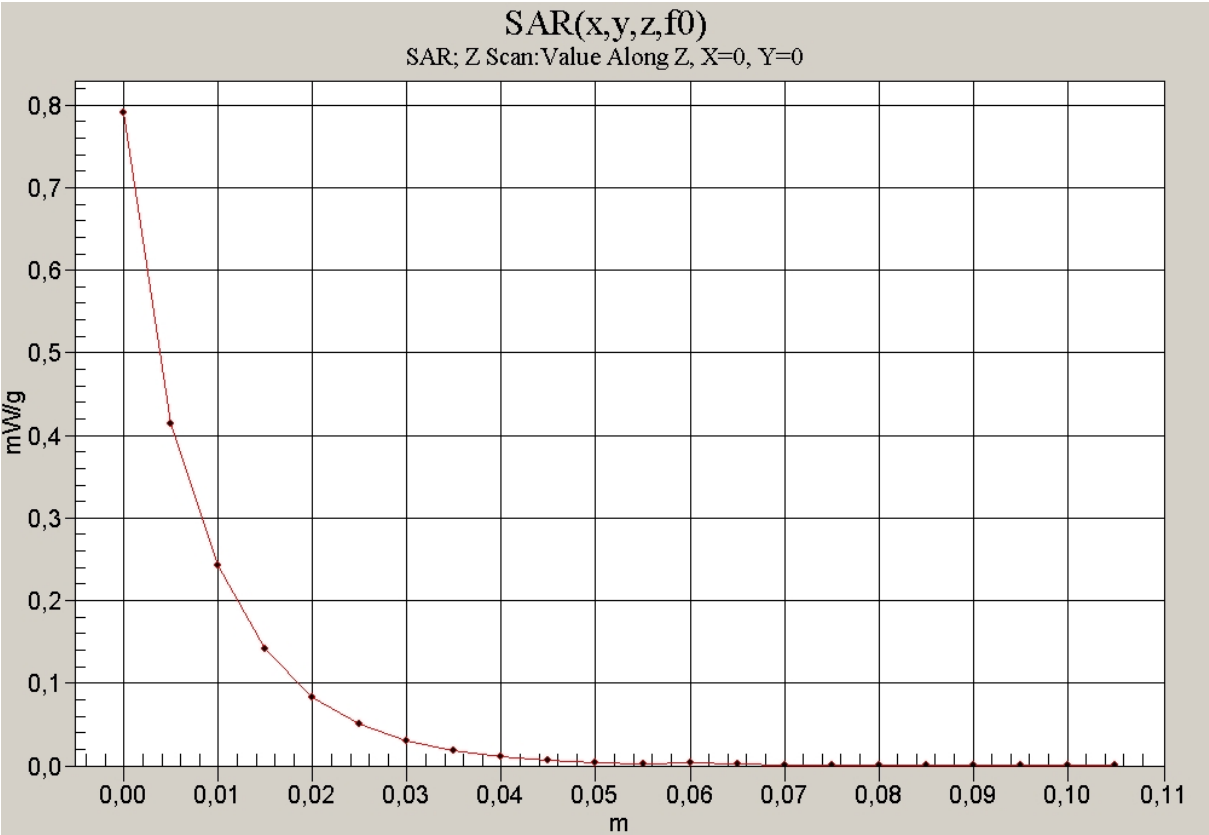
1900 MHz head
