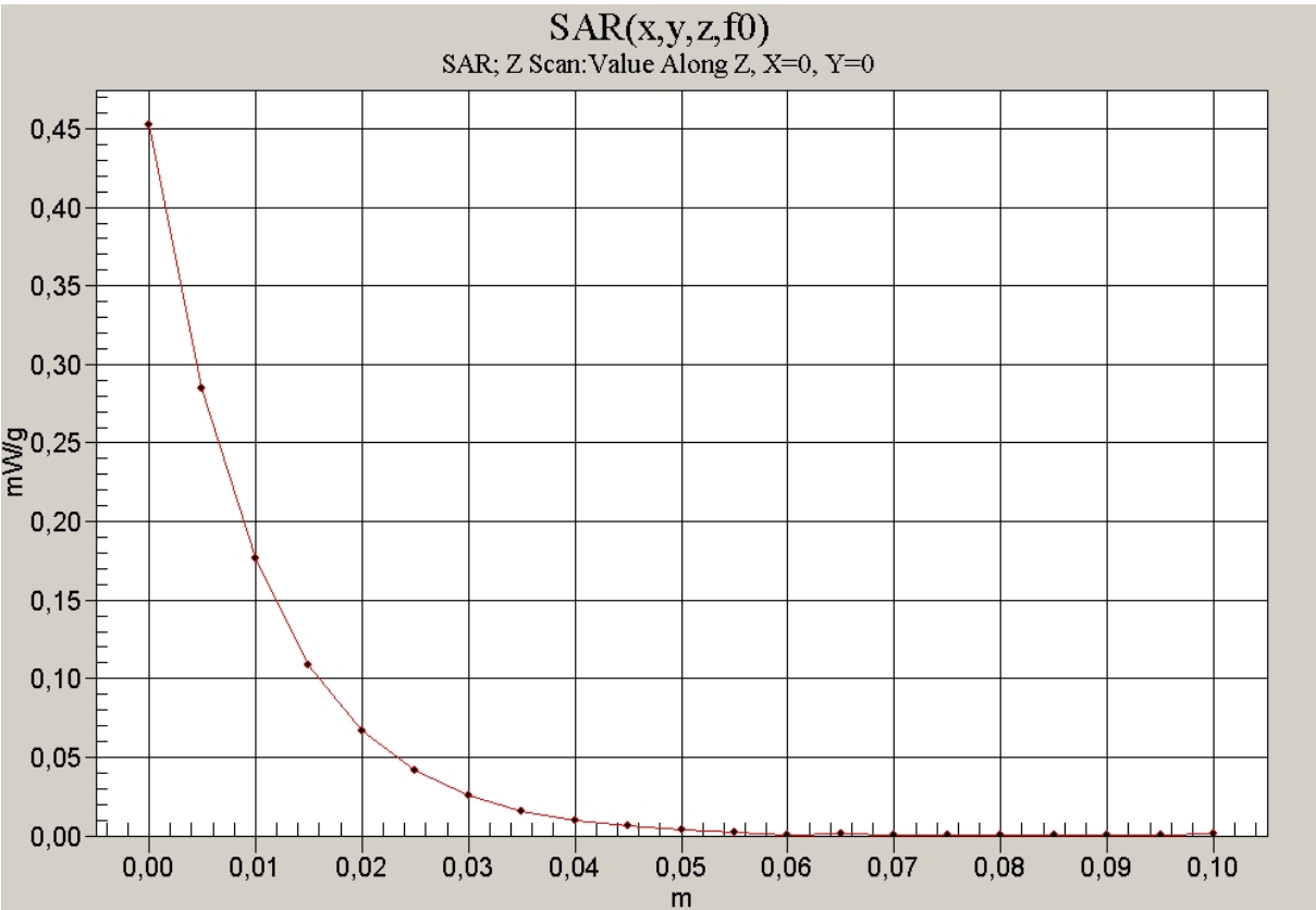
1900 MHz body
