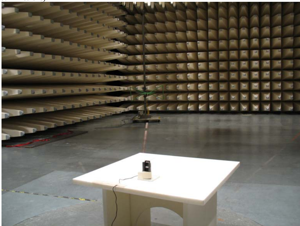
Photo 1 (Radiated Emissions):
