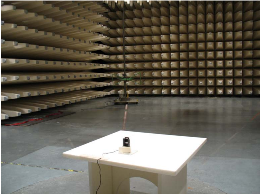
Photo 1: Radiated Emissions
