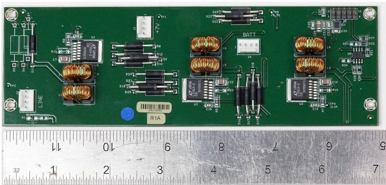
IWT GWN Power Supply Board Top View
