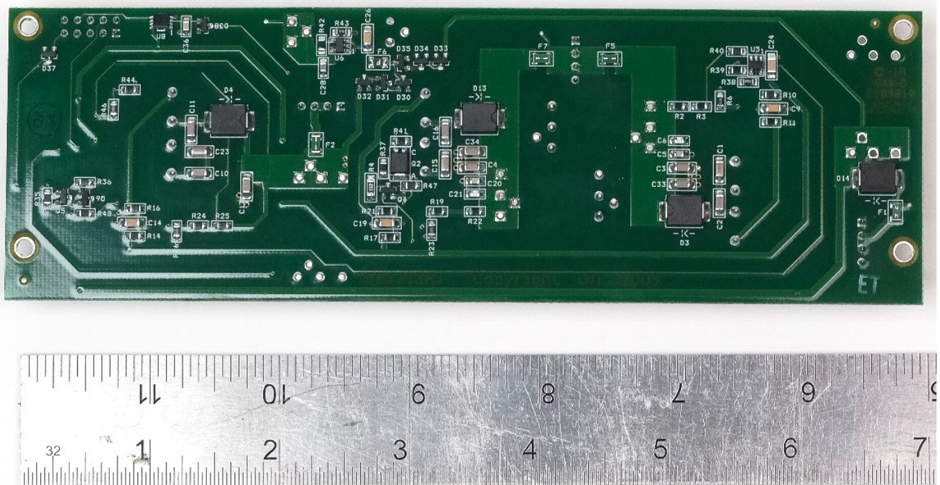
IWT GWN Power Supply Board Bottom View
