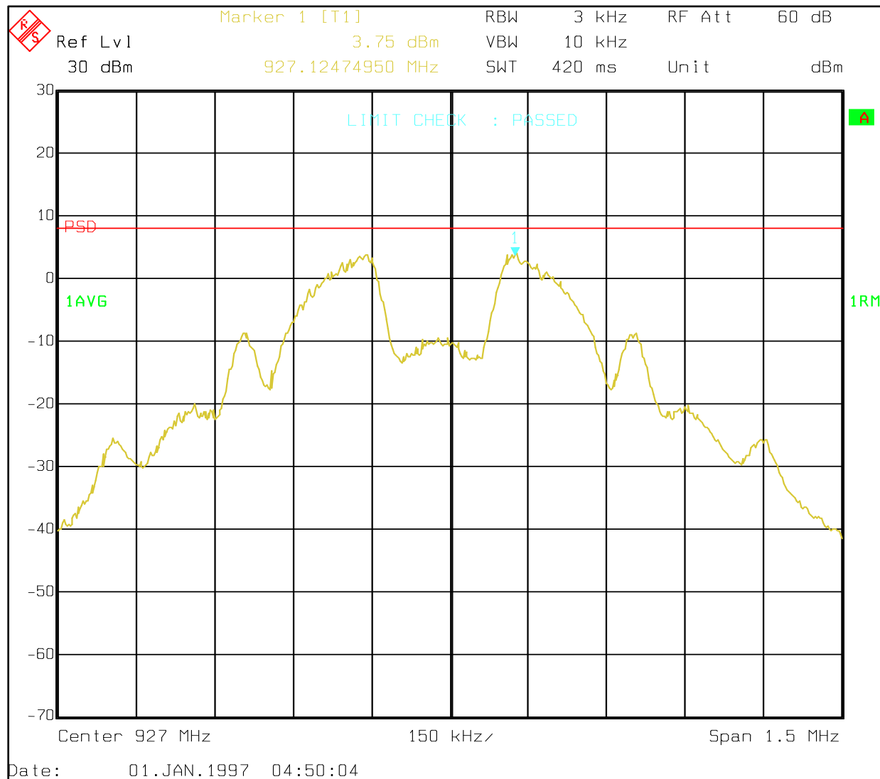
Plot 7-3: Power Spectral Density – 927 MHz
