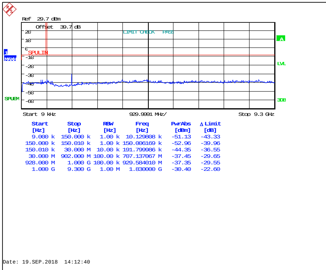
Plot 5-2: Antenna Conducted Spurious Emissions (915 MHz)
