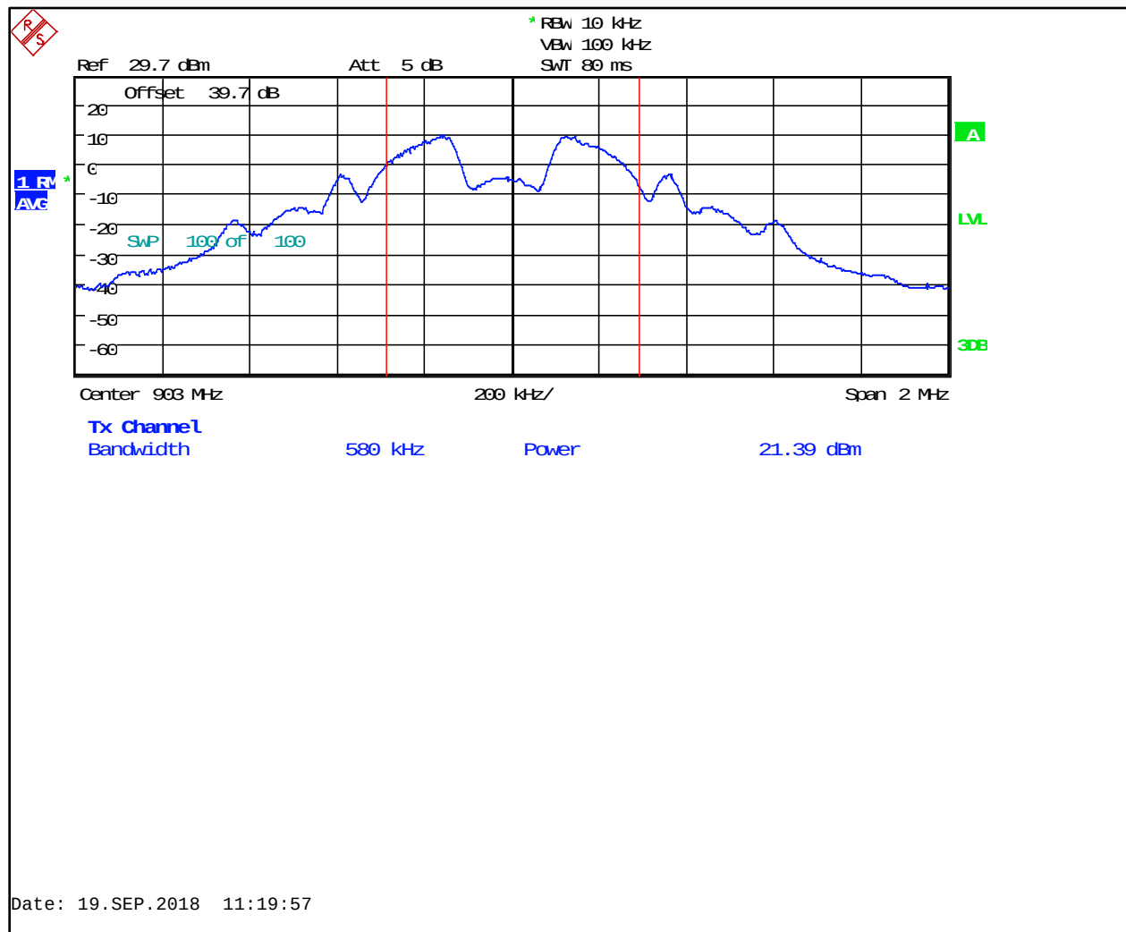
Plot 3-1: Maximum Conducted Output Power (903 MHz)
