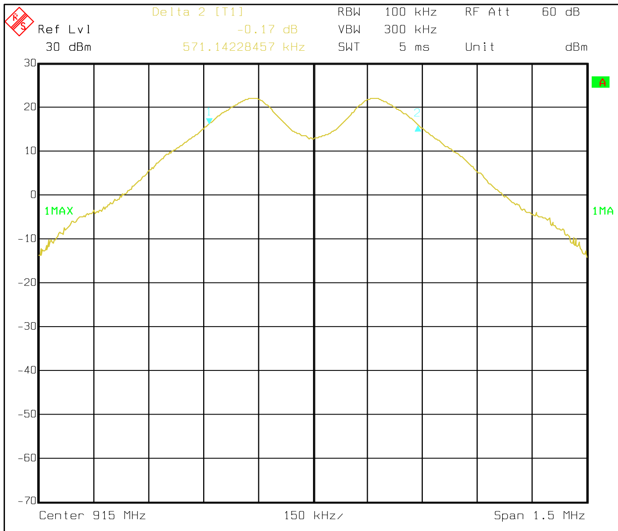
Plot 6-2: 6 dB Bandwidth – 915 MHz
