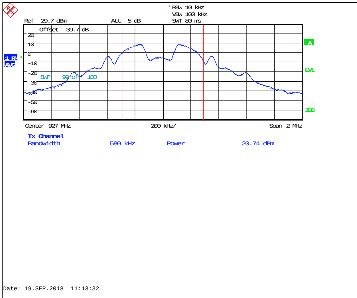
Plot 3-3: Maximum Conducted Output Power (927 MHz)
