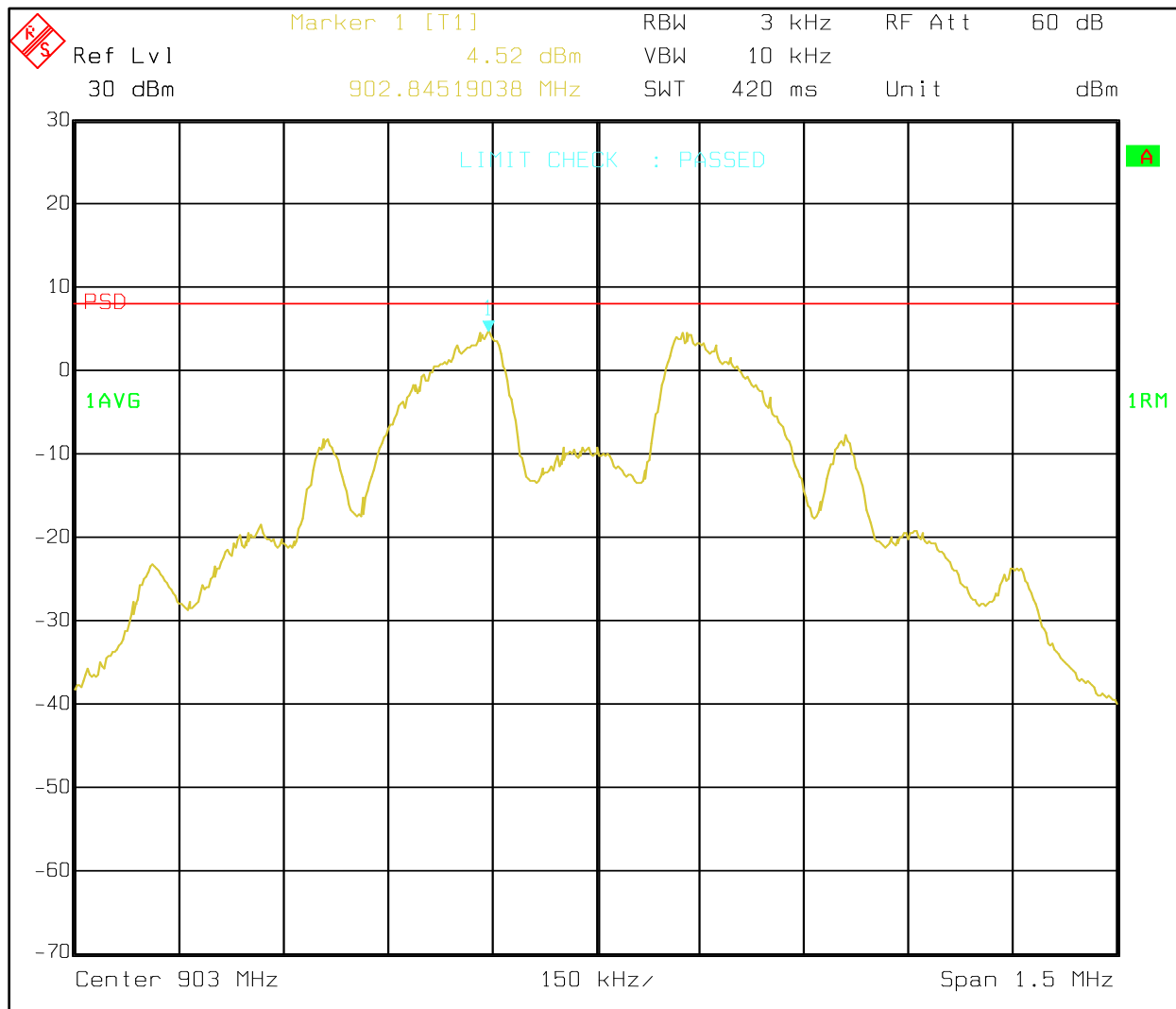
Plot 7-1: Power Spectral Density – 903 MHz
