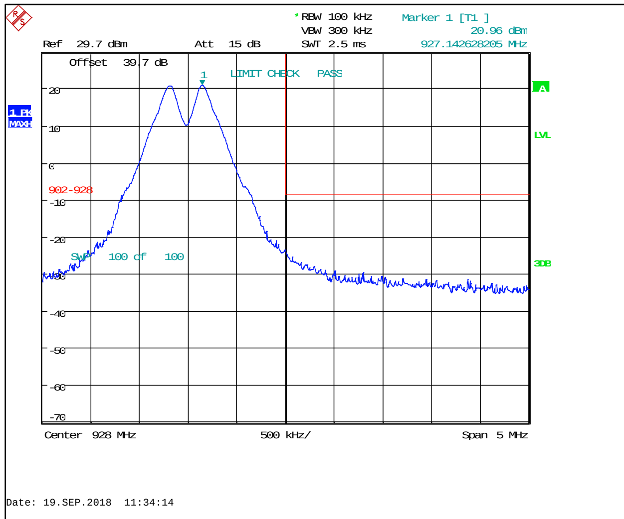
Plot 4-2: Upper Band Edge (928 MHz Band Edge, 927 MHz Carrier)
