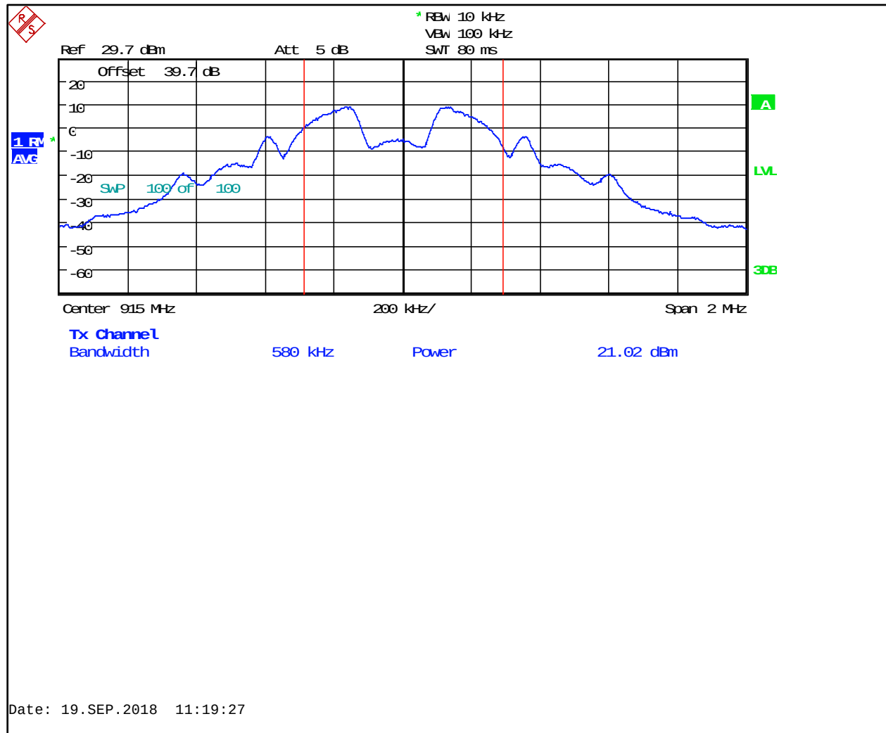
Plot 3-2: Maximum Conducted Output Power (915 MHz)
