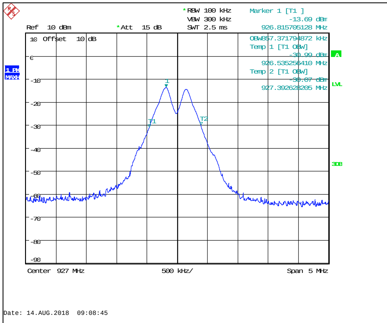
Plot 6-6: 99% Bandwidth – 927 MHz
