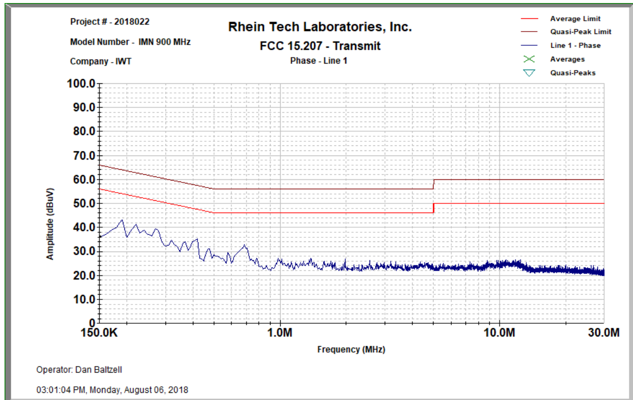
Plot 8-3: Conducted Line Emissions – Phase – Transmit Mode
