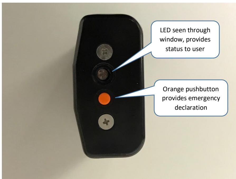
Figure 4 - Front Side View of Tracking Tag
