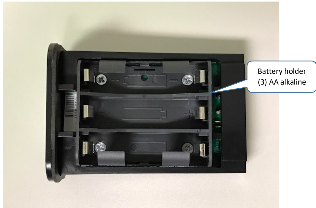
Figure 9 - Bottom side of interior 'Tray' with battery holder
