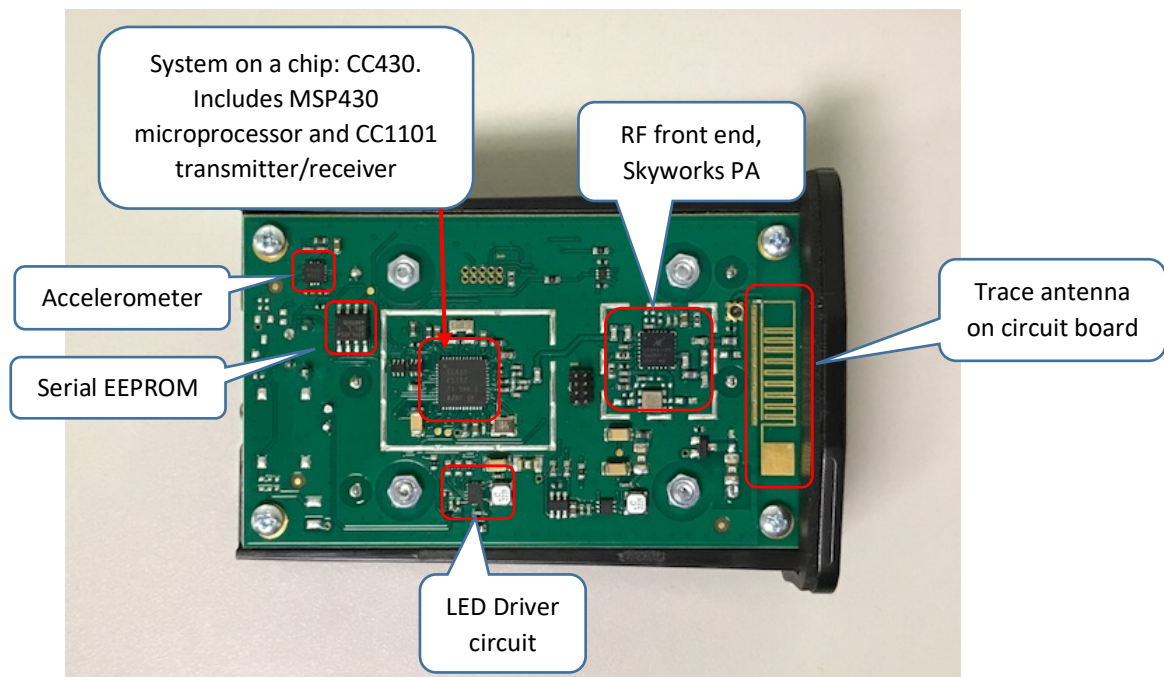
Figure 8 - Top View of Circuit Board
