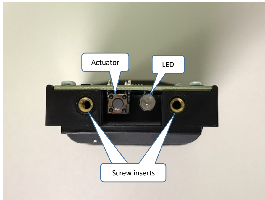
Figure 10 - Front view of interior 'Tray' with battery holder. Actuator and LED are mounted on edge of circuit board
