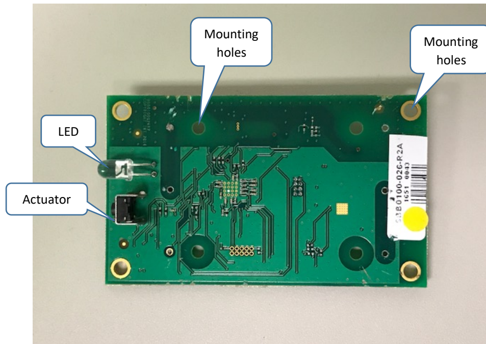
Figure 11 - Bottom View of Circuit Board
