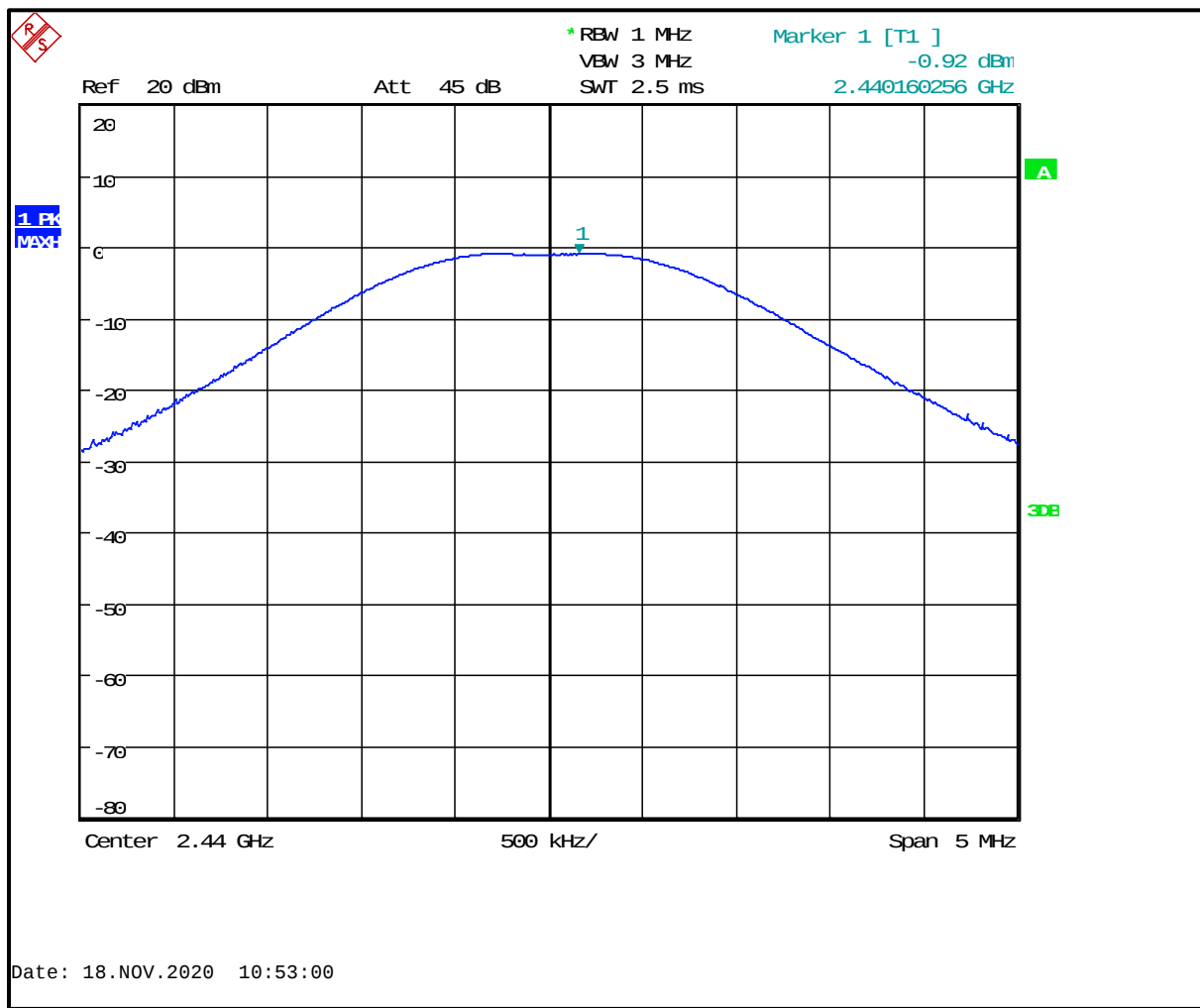
Plot 3-2: Maximum Conducted Output Power (2440 MHz)
