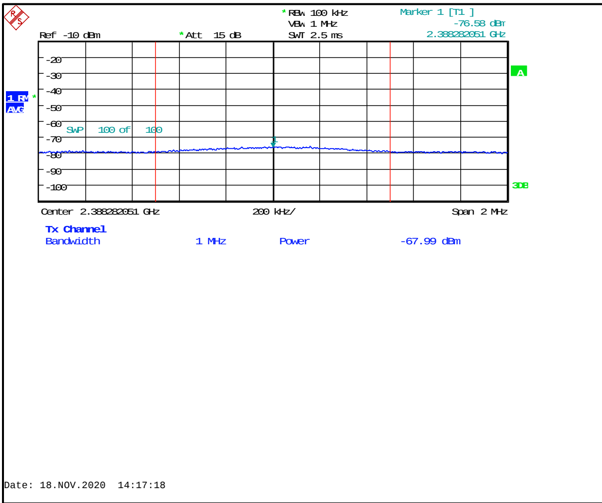
Plot 4-2: Lower Band Edge (Average, 2402 MHz Carrier)
