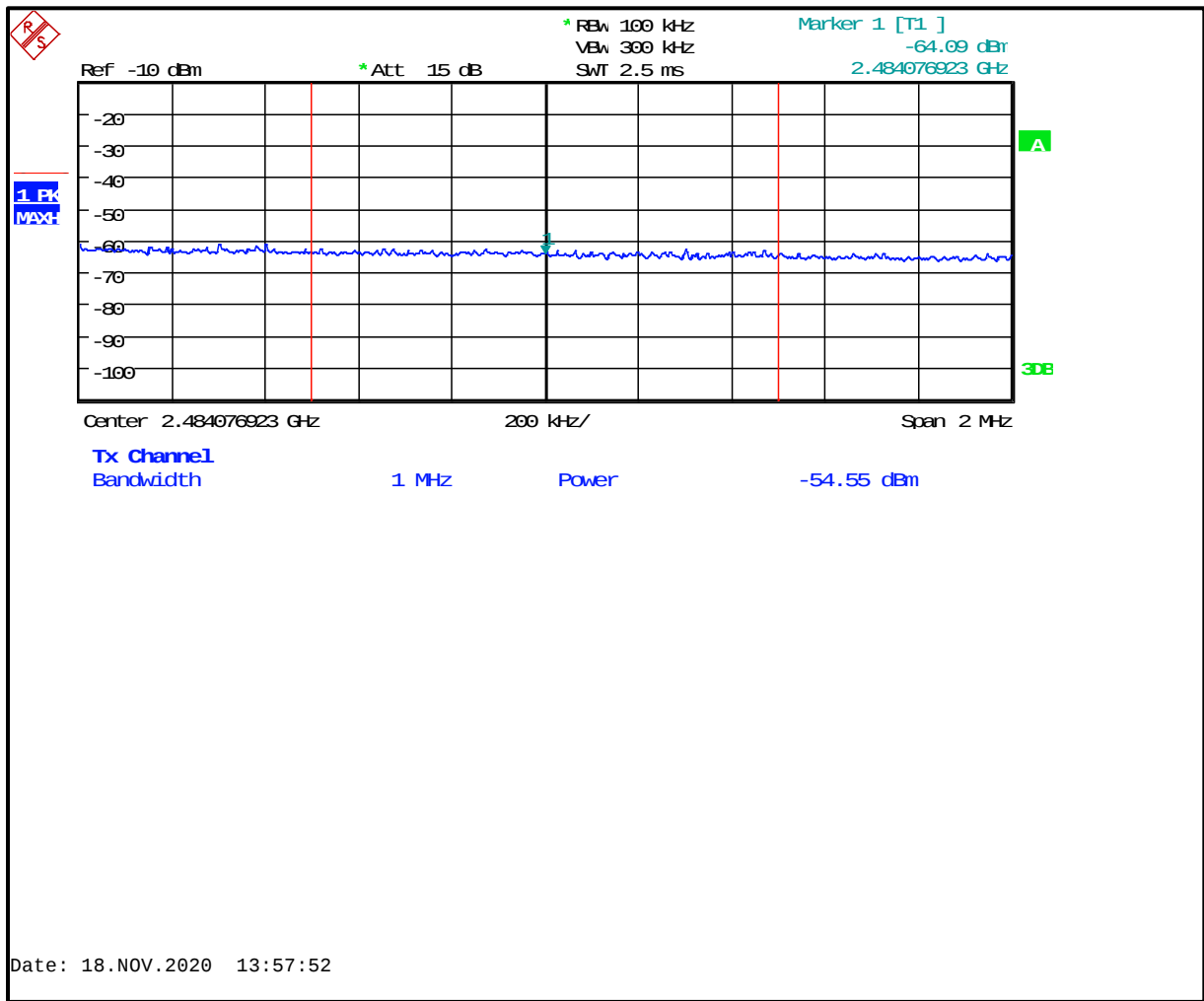
Plot 4-3: Upper Band Edge (Peak, 2480 MHz Carrier)
