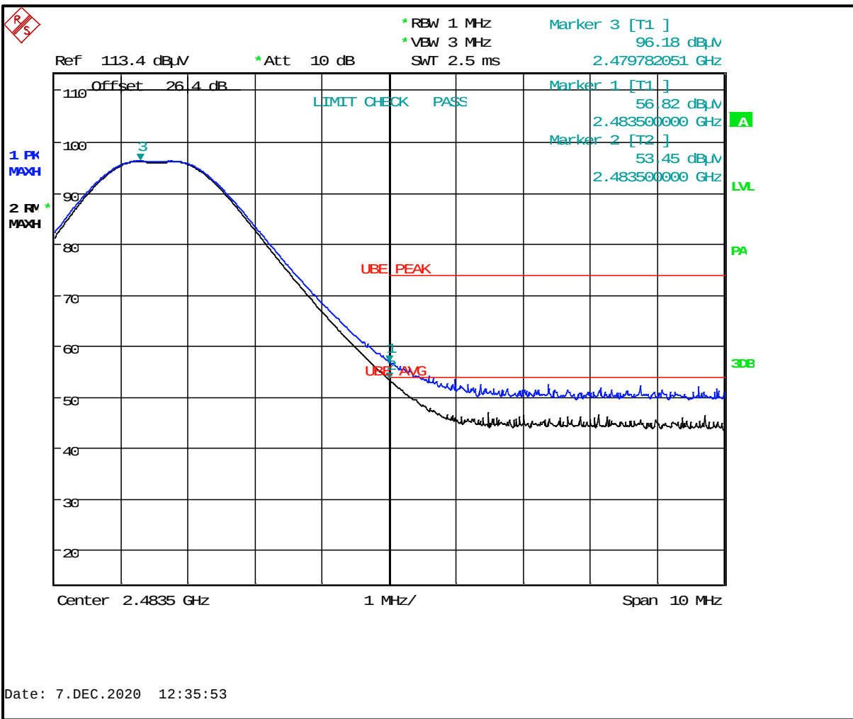
Plot 9-1: Restricted Upper Band Edge (Peak and Average, 2480 MHz Carrier)
