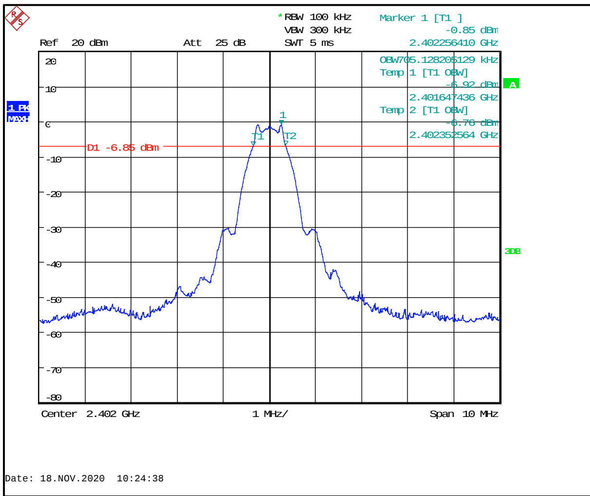
Plot 6-1: 6 dB Bandwidth – 2402 MHz
