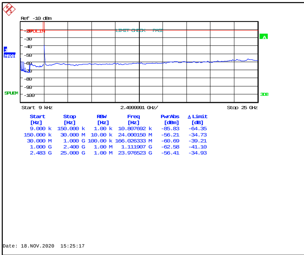
Plot 5-3: Antenna Conducted Spurious Emissions (2480 MHz)
