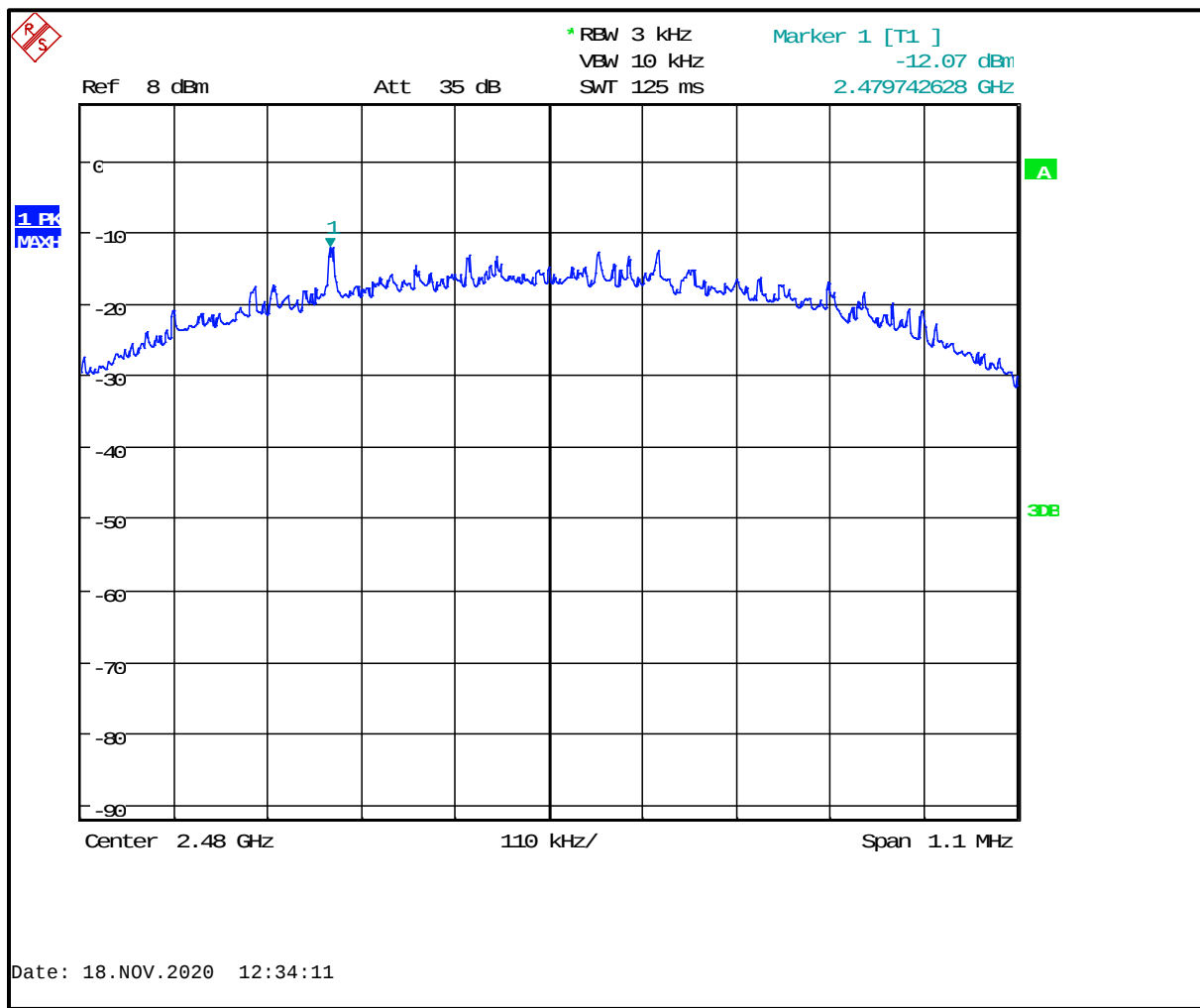
Plot 7-3: Power Spectral Density – 2480 MHz
