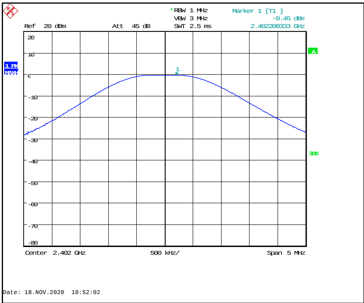
Plot 3-1: Maximum Conducted Output Power (2402 MHz)
