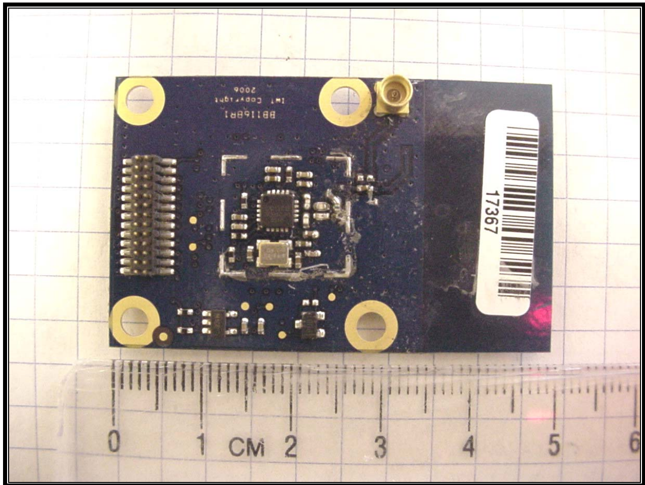
Photograph 7: Bottom of PCB without Shield
