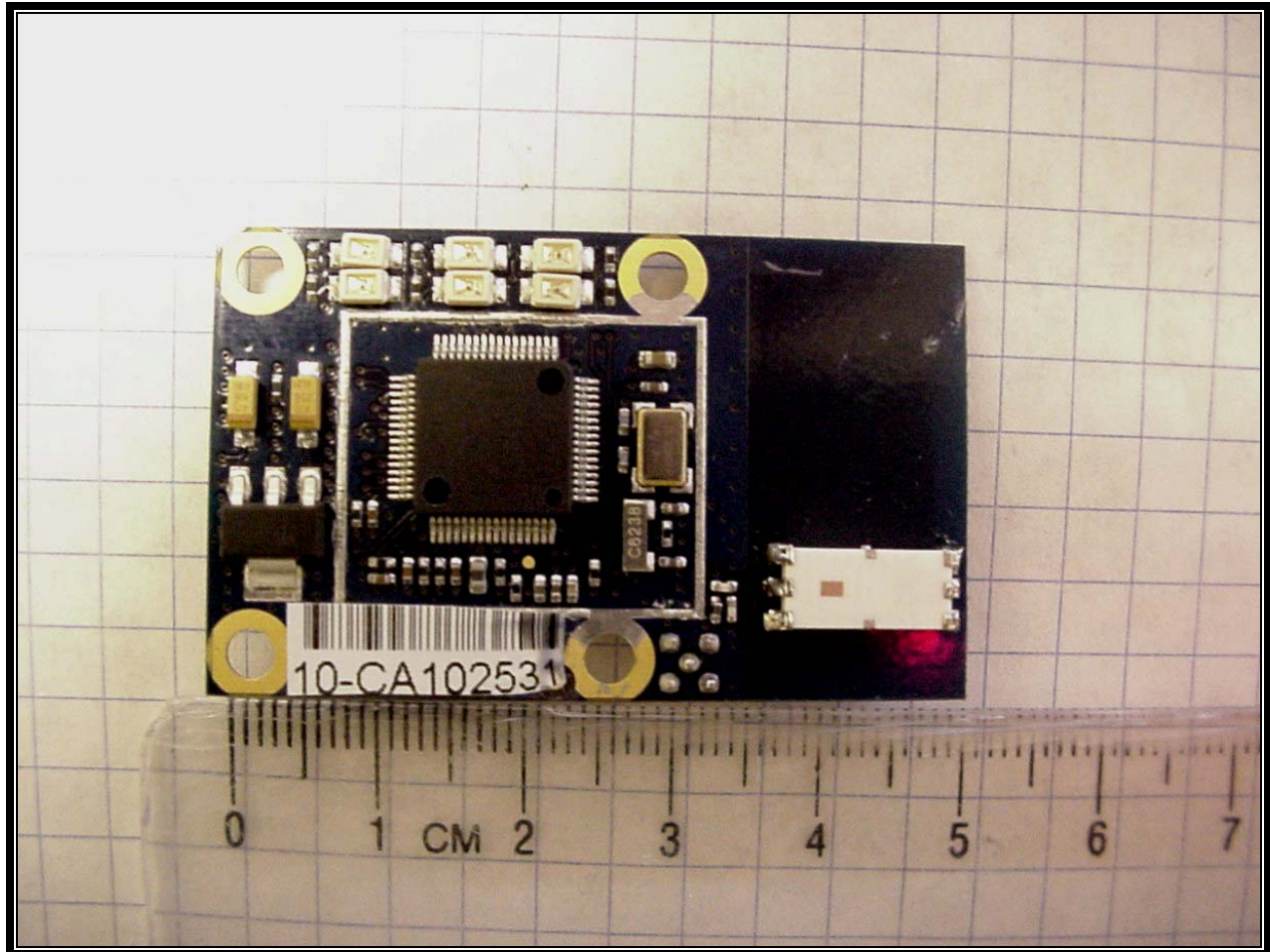
Photograph 5: Top of PCB
