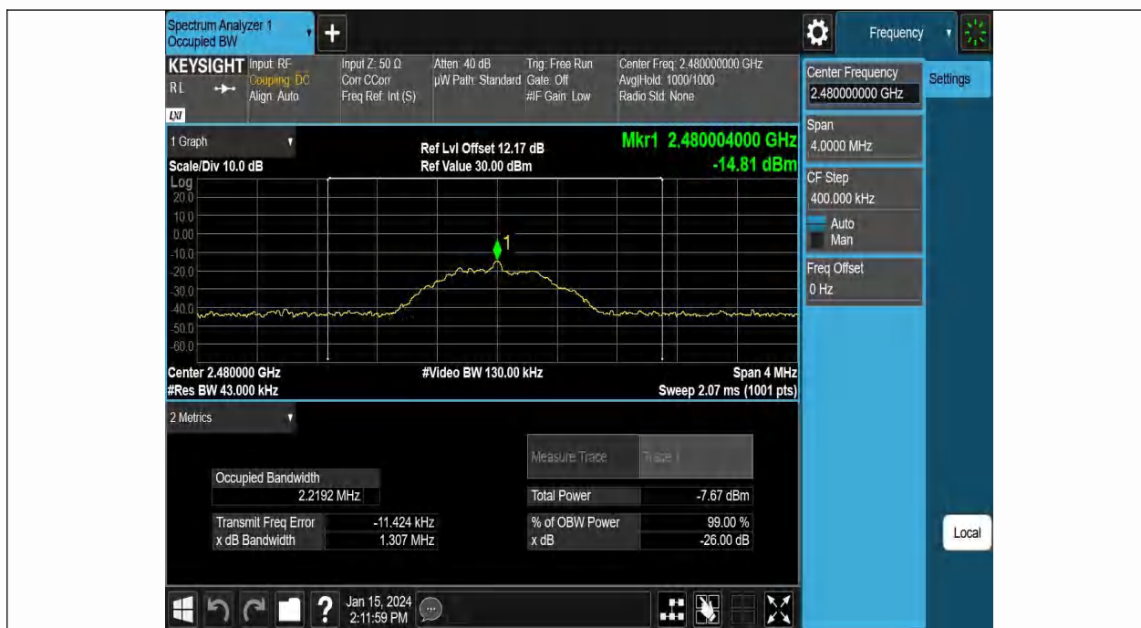
BLE_1M-Ant1-2480
