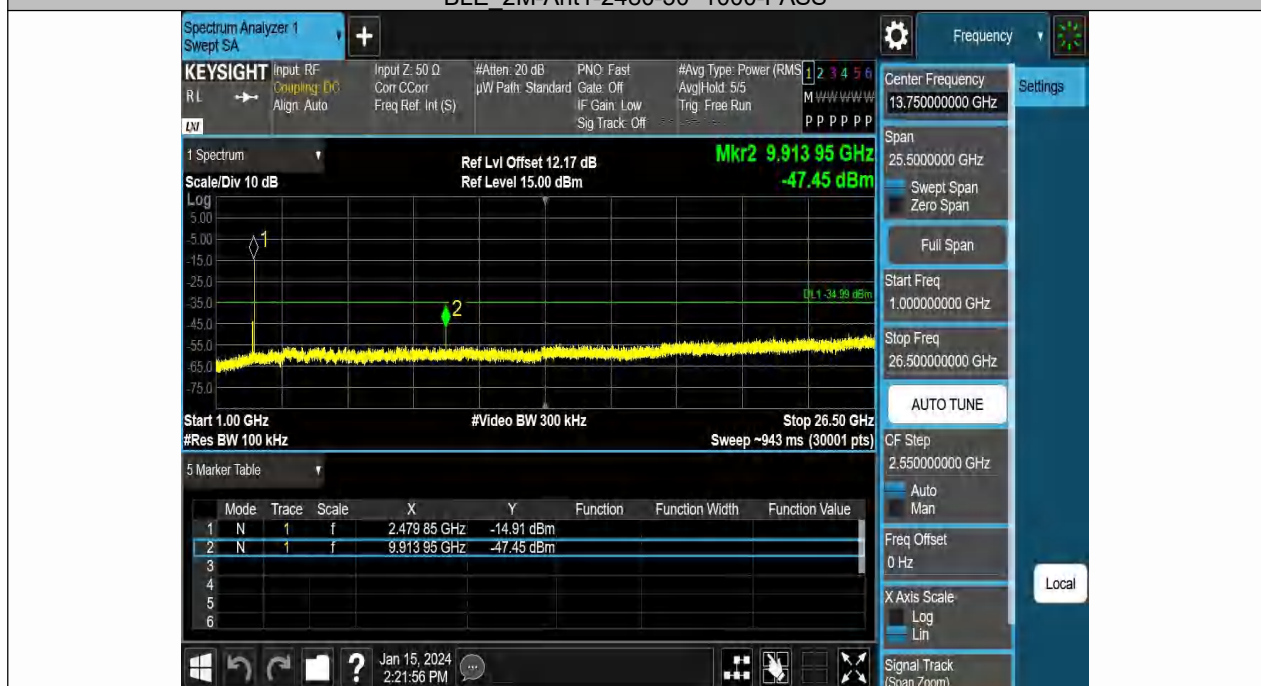
BLE_2M-Ant1-2480-1000~26500-PASS
