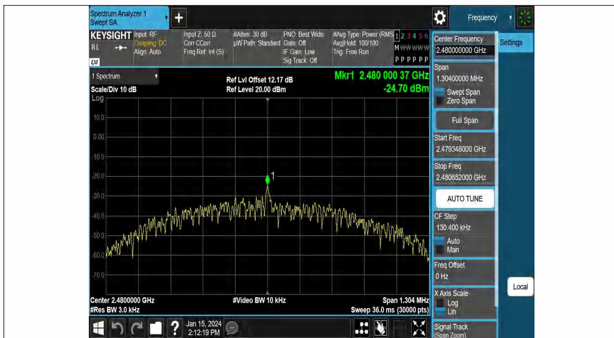
BLE_1M-Ant1-2480-PASS
