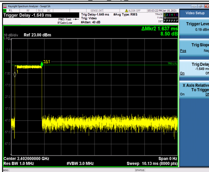
2DH3_Ant1_Hop_2402
