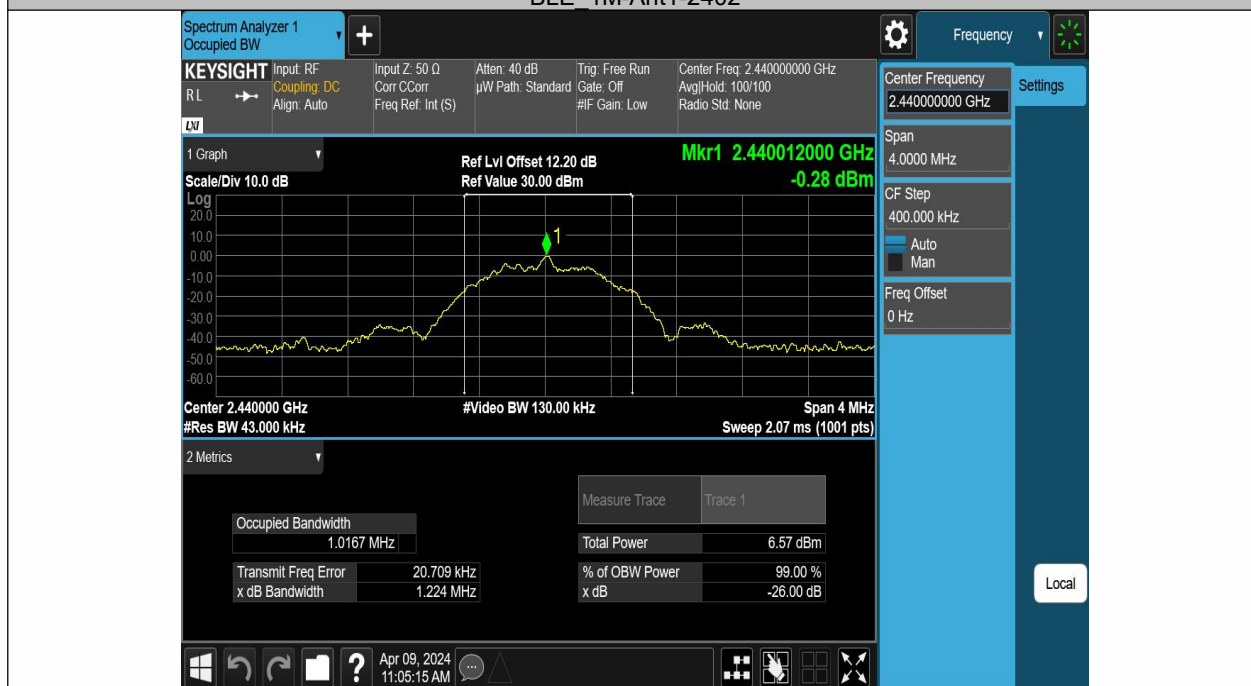
BLE_1M-Ant1-2440
