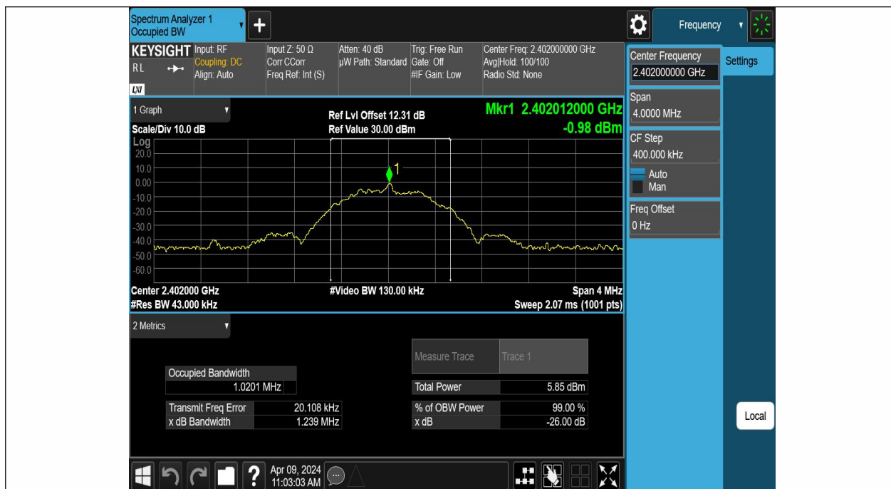
BLE_1M-Ant1-2402
