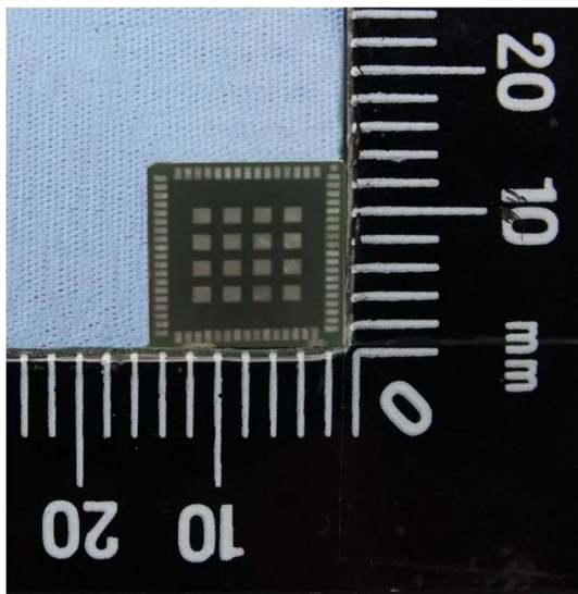
Bottom View of 60-SIPT BT-WiFi Module
