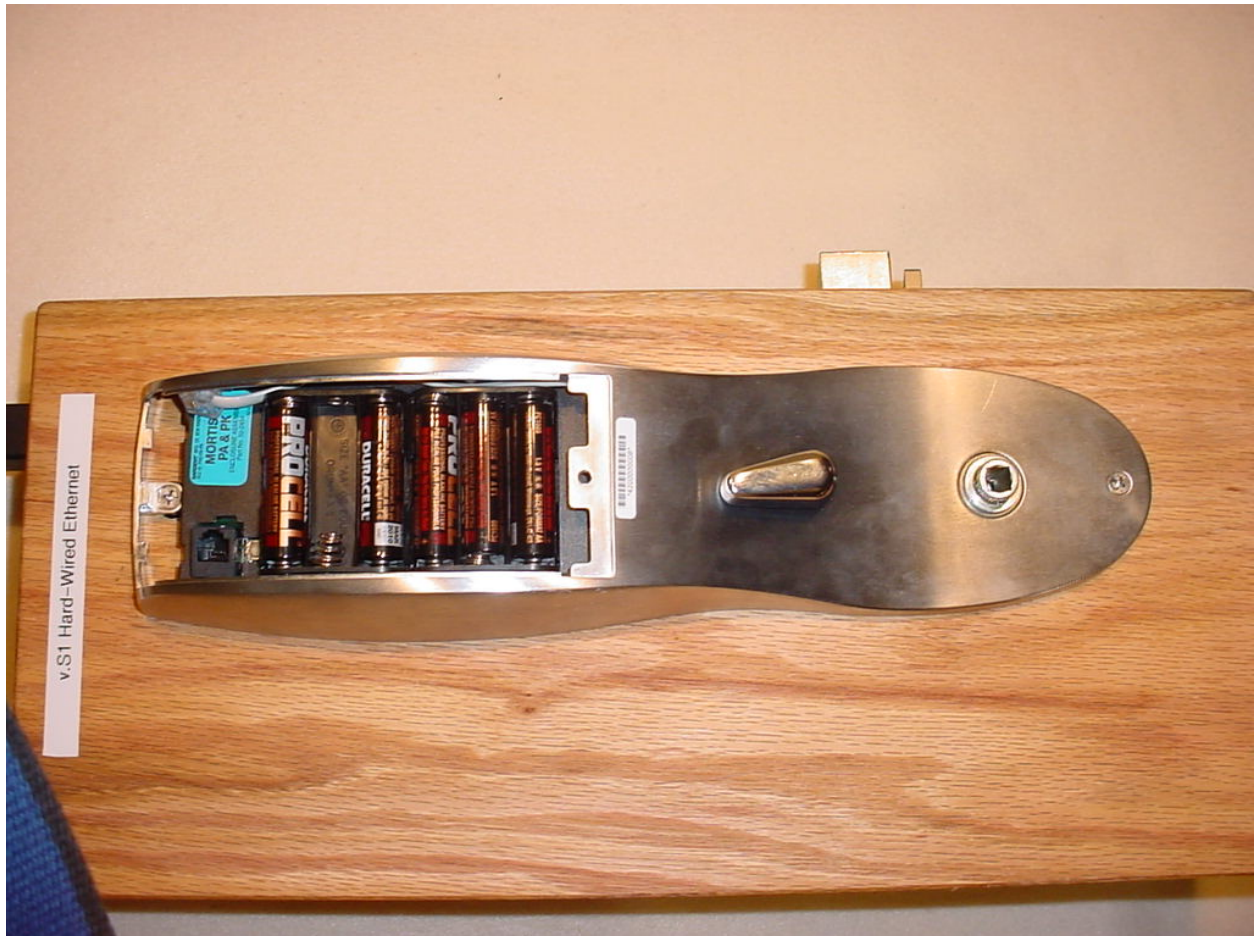
Figure 2: Low Profile Enclosure (Rear View)
