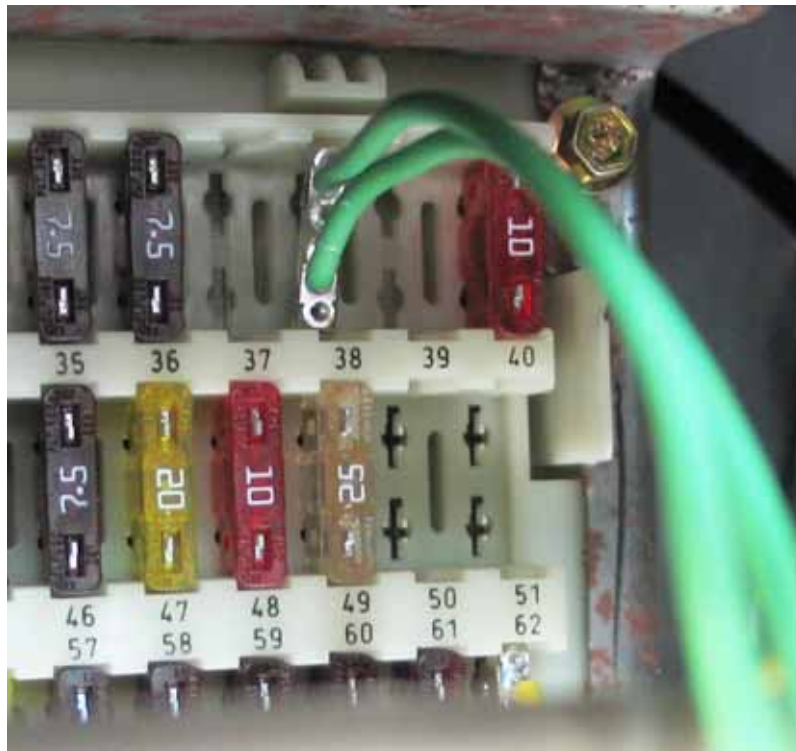
Figure 3. Attached Ignition Cable
