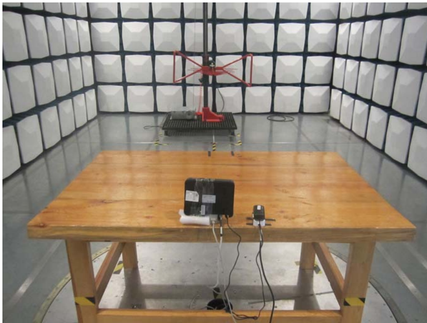
Radiated Emission 30MHz-1000MHz – Rear View
