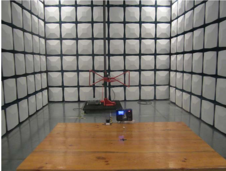
Radiated Emission 30MHz-1000MHz – Front View
