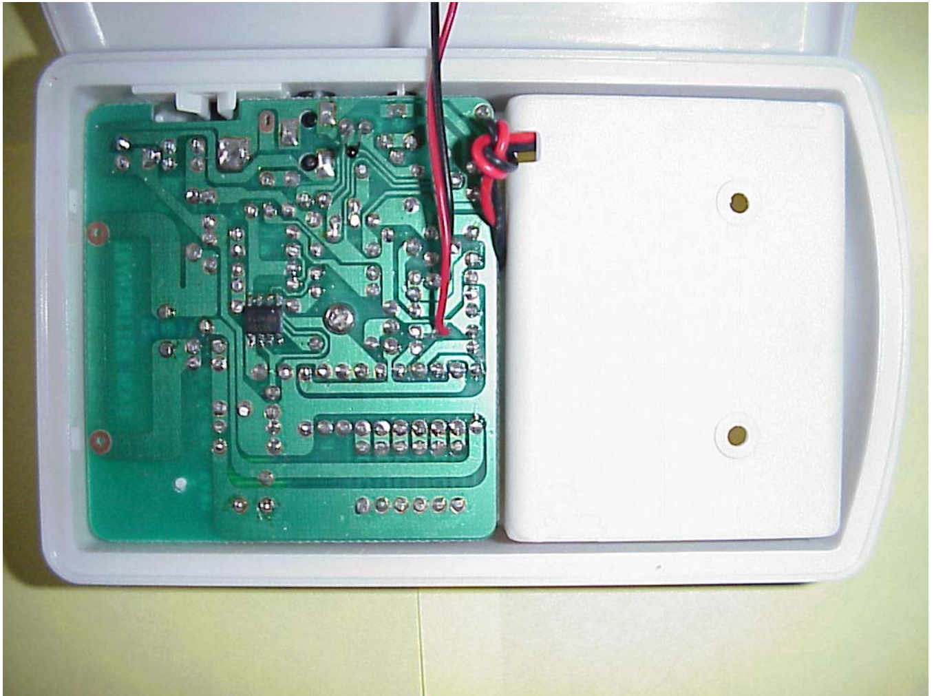
BOTTOM SIDE OF TRANSMITTER CIRCUIT BOARD
