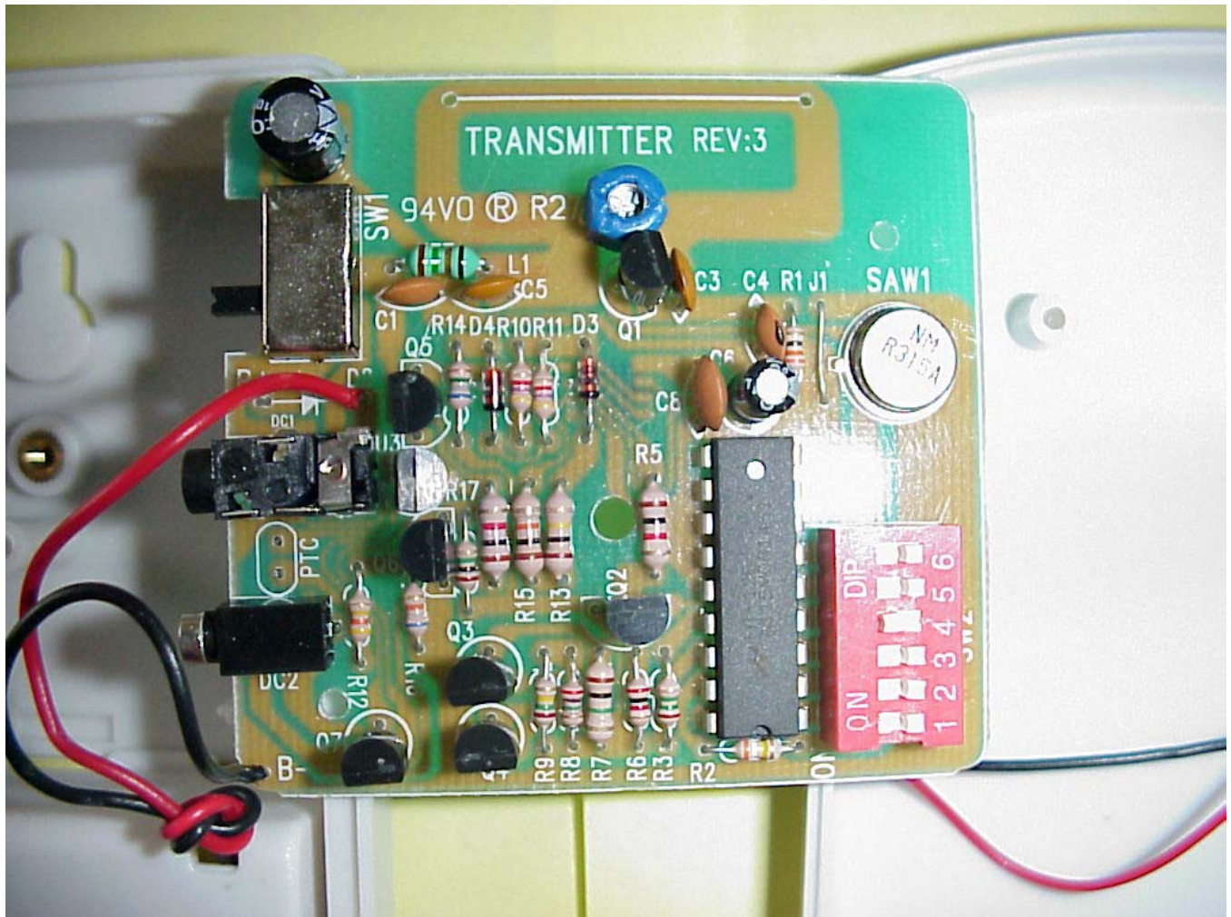
CLOSE UP OF TRANSMITTER CIRCUIT BOARD
