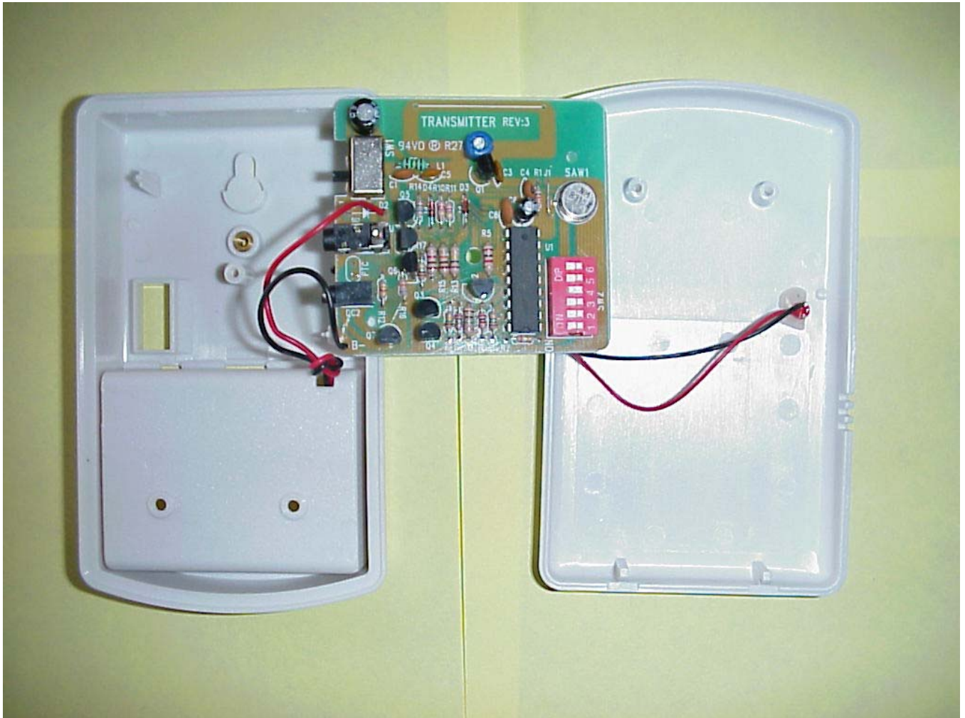
TOP SIDE OF TRANSMITTER CIRCUIT BOARD
